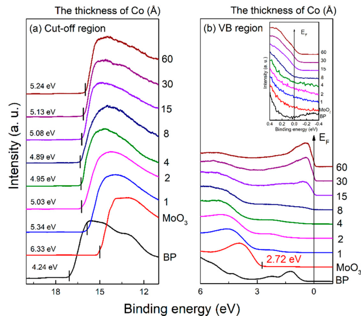
Figure 2. UPS spectra as a function of Co film thickness when growing Co thin films on \text{MoO}_3/\text{BP} , (a) cut-off region, (b) VB region, Inset: the locally enlarged view of the VB edge region near E_F .
