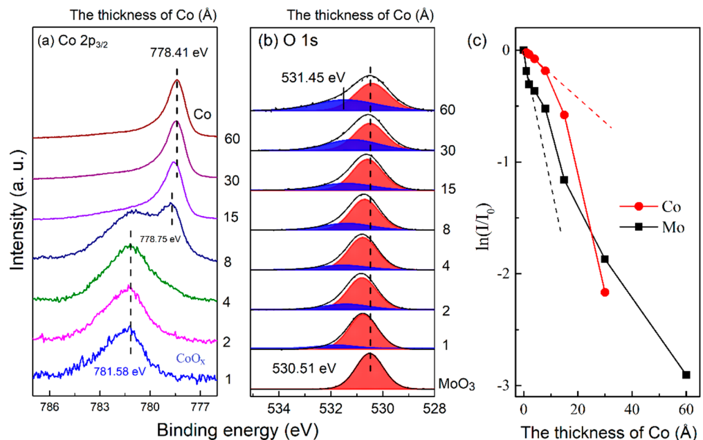
Figure 3. XPS spectra as a function of Co film thickness when growing Co thin films on \text{MoO}_3/\text{BP} . (a) Co 2p, (b) O 1s, the blue (red) peak corresponds to the oxygen component in \text{CoO}_x ( \text{MoO}_3 ). (c) Photoelectron intensity as a function of Co film thickness. The red (black) dashed line marks the slope of Co 2p (Mo 3d) before Co deposition to 8 \text{ \AA} .
