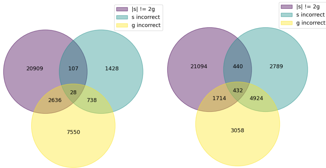
Figure 5: Comparing the number of s -invariants and slice genres predicted incorrectly by neural networks with the number of cases where the slice genus saturates the lower bound provided by the s -invariant. Left figure is trained on the Khovanov polynomial and right figure is trained on the Jones polynomial.
