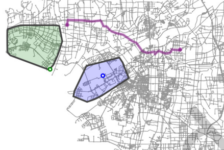
Fig. 6. Initialization: Use discovered path as basis route (purple line) for the next level
