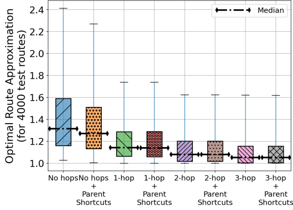
Fig. 11. Distribution of Optimal Route Approximation results for different Shortcut Connection methods
