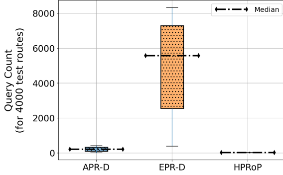
Fig. 18. Distribution of the required number of queries for route completion
