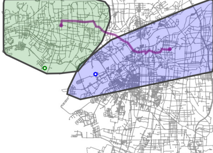
Fig. 5. Initialization: Find a shortest path between the lowest-level partitions containing s (blue circle) and d (green) separately.
