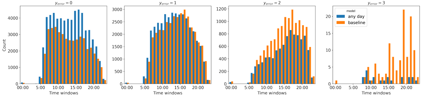
Fig. 7. Comparison between baseline and any day trip level models. From left to right, the plots show the counts of mean absolute error, y_{error} = \{0, 1, 2, 3\} , of the predicted to the true label. The model is able to provide 40% more correct predictions and 29% less mistakes than the baseline.
