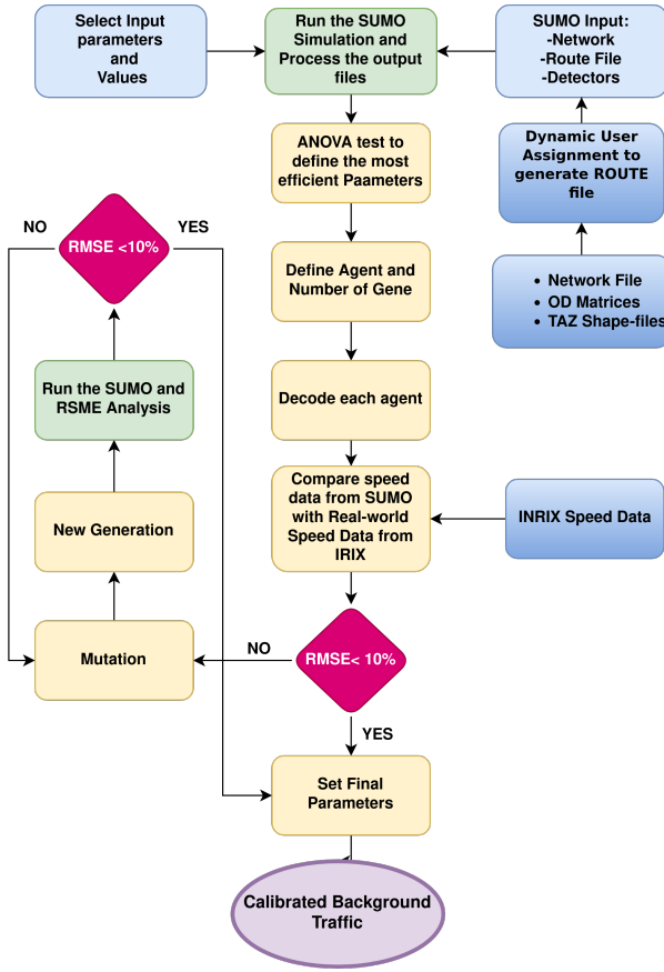
Fig. 3: Calibration procedure
