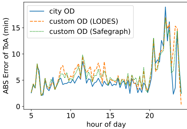
Fig. 9: BTE-Sim for different OD data
