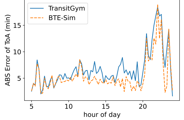
Fig. 7: Comparing Transit-gym and BTE-Sim on absolute error of Time of Arrival
