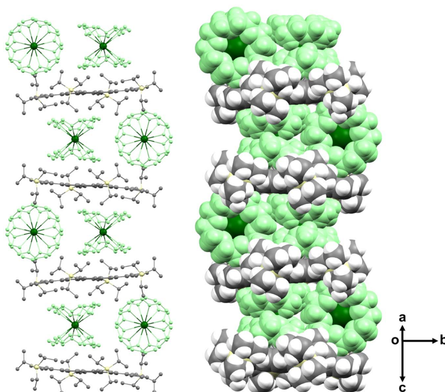
Fig. 7 Solid-state packing of [(Cs^+(18\text{-crown-6})_2)_2(2a^{2-})] in ball-and-stick (no H-atoms, left) and space-filling (right) models. The \{Cs^+(18\text{-crown-6})_2\} moieties are shown in green.
