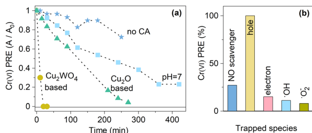
Fig. 5 \text{Cr}(\text{vi}) photoreduction with CBTO under excitation with 100 \text{ mW cm}^{-2} light, 40 \text{ mL} of 5 \text{ mg L}^{-1} \text{Cr}(\text{vi}) solution, 10 \text{ mM} CA, \text{pH} = 2 unless stated otherwise (a) depending on synthesis technique, pH, and (b) presence of citric acid PRP at 240 min in the presence of different scavengers (CBTO: 200 \text{ mg L}^{-1} ).
