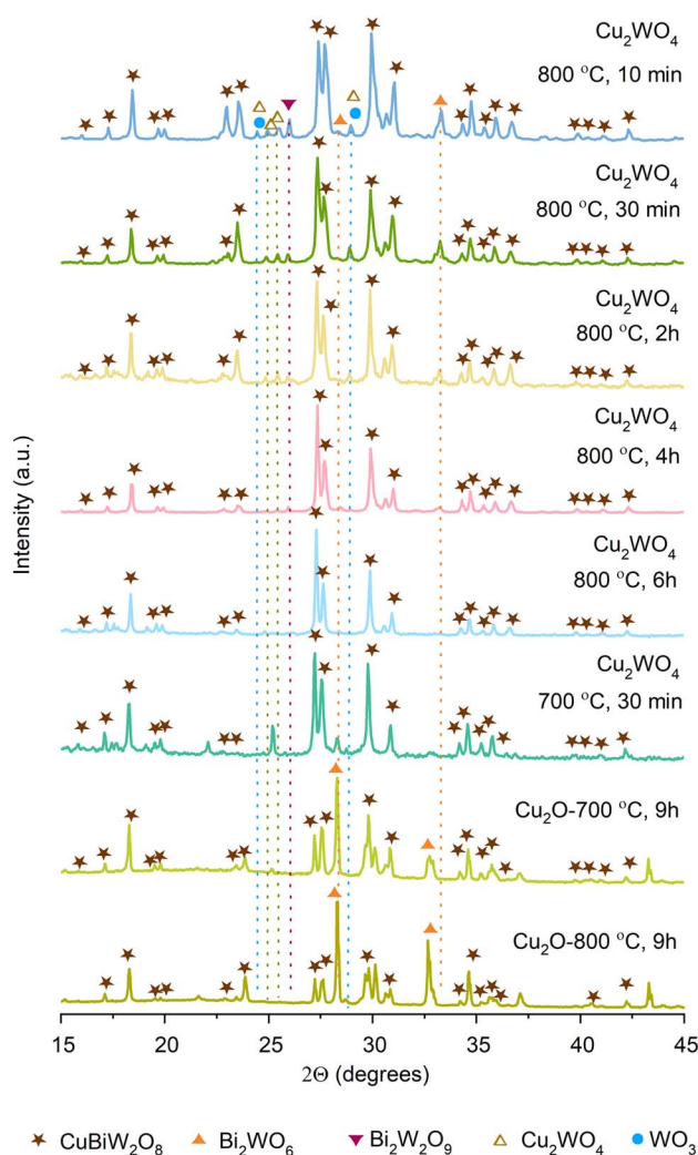
Fig. 3 XRD diagrams showing \text{Cu}_2\text{WO}_4 based CBTO synthesis at varying temperatures and durations in Cu rich environment under argon compared with \text{Cu}_2\text{O} based synthesis.
