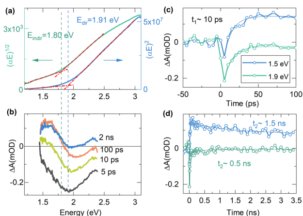
Fig. 4 Optical properties of CBTO (a) Tauc plot for determining the indirect (1.80 eV) and direct (1.91 eV) band gaps. (b) Transient absorption spectra recorded at different times after excitation with 76.4\ \mu\text{J}\ \text{cm}^{-2} , 450 nm (2.76 eV) optical pulses. Transient absorption kinetics at 1.5 eV and 1.9 eV over early (c) and long (d) time scales.
