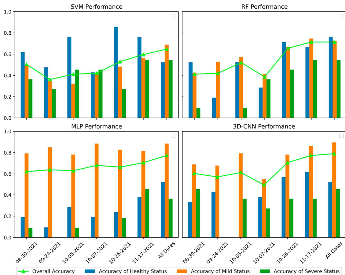
Figure 8. The overall accuracy (OA) and accuracy of each class as a result of support vector machine (SVM), random forest (RF), multilayer perceptron (MLP), and 3D convolutional neural network (3D-CNN) over temporal datasets (date format: MM/DD/YYYY).
