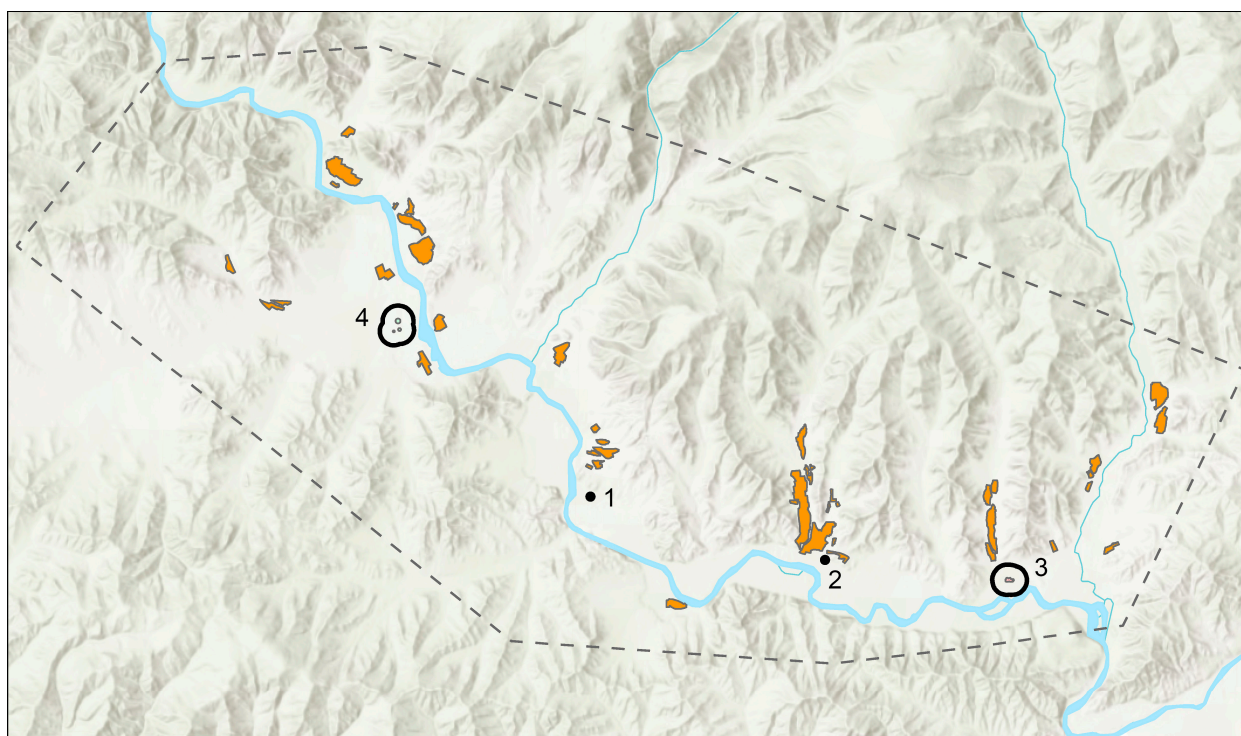
Figure 2. Map of the Egiin Gol valley region with study area marked by dashed outline and relict agricultural fields in brown. Xiongnu settlements discussed are as follows: 1. EGS 486; 2. EGS 110; 3. EGS 36 with perimeter; 4. EGS 297-99 with perimeter (Basemap Credit: Esri, Intermap, NASA, NGA, USGS).
