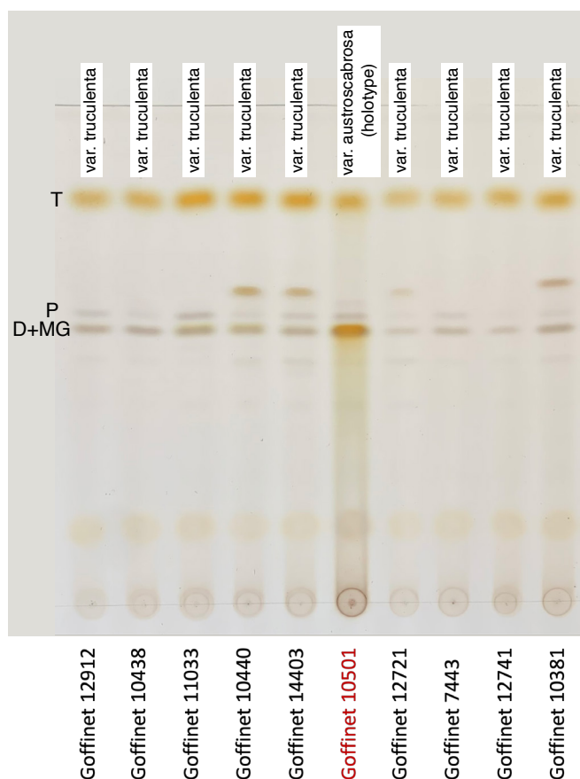
Fig. S3 TLC in phase C for representatives of P. triculenta (incl. var. austroscabrosa ). See Table S2 for detailed voucher information. D = dolichorrhizin, G = gyrophoric acid, M = methylgyrophorate, P = peltidactylin, T = tenuiorin, Z = zeorin. See Material and Methods for details.
