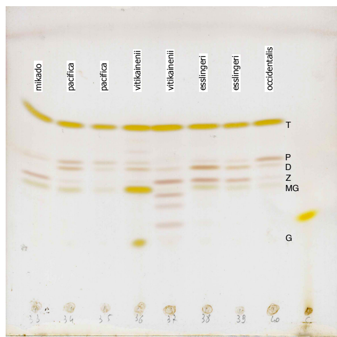
Fig. S7 TLC in phase C for representatives of the pacifica group and occidentalis subclade. See Table S2 for detailed voucher information. D = dolichorrhizin, G = gyrophoric acid, M = methylgyrophorate, P = peltidactylin, T = tenuiorin, Z = zeorin. See Material and Methods for details.
