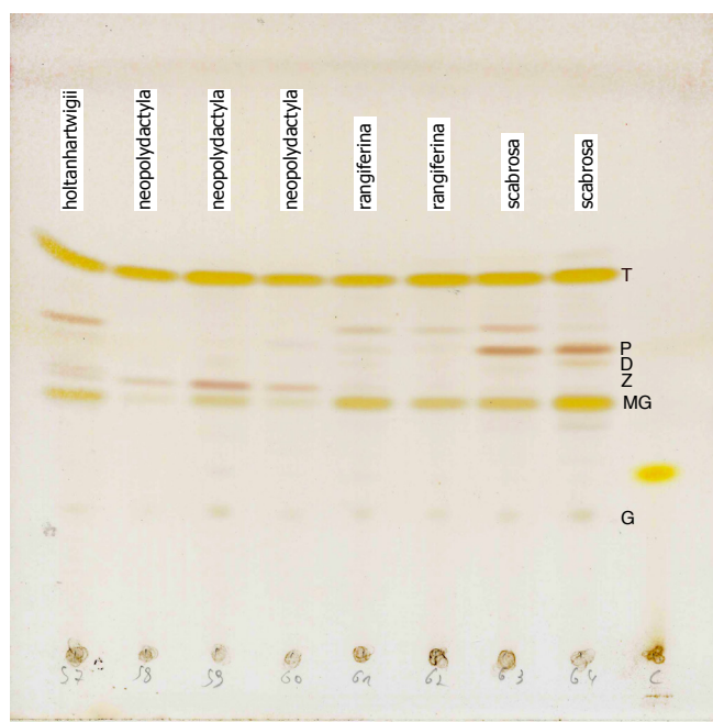
Fig. S10 TLC in phase C for representatives of the scabrosa subclade. See Table S2 for detailed voucher information. D = dolichorrhizin, G = gyrophoric acid, M = methylgyrophorate, P = peltidactylin, T = tenuiorin, Z = zeorin. See Material and Methods for details.
