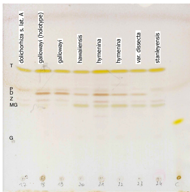
Fig. S4 TLC in phase C for representatives of Peltigera hawaiiensis and P. gallowayi . See Table S2 for detailed voucher information. D = dolichorrhizin, G = gyrophoric acid, M = methylgyrophorate, P = peltidactylin, T = tenuiorin, Z = zeorin. See Material and Methods for details.
