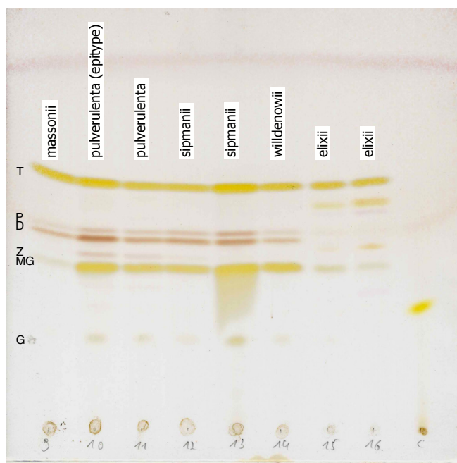
Fig. S2 TLC in phase C for representatives of the dolichorhiza and hymenina groups. See Table S2 for detailed voucher information. D = dolichorrhizin, G = gyrophoric acid, M = methylgyrophorate, P = peltidactylin, T = tenuiorin, Z = zeorin. See Material and Methods for details.
