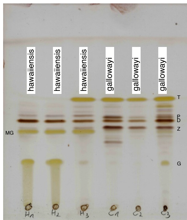
Fig. S5 TLC in phase C for representatives of the hymenina group. See Table S2 for detailed voucher information. D = dolichorrhizin, G = gyrophoric acid, M = methylgyrophorate, P = peltidactylin, T = tenuiorin, Z = zeorin. See Material and Methods for details.
