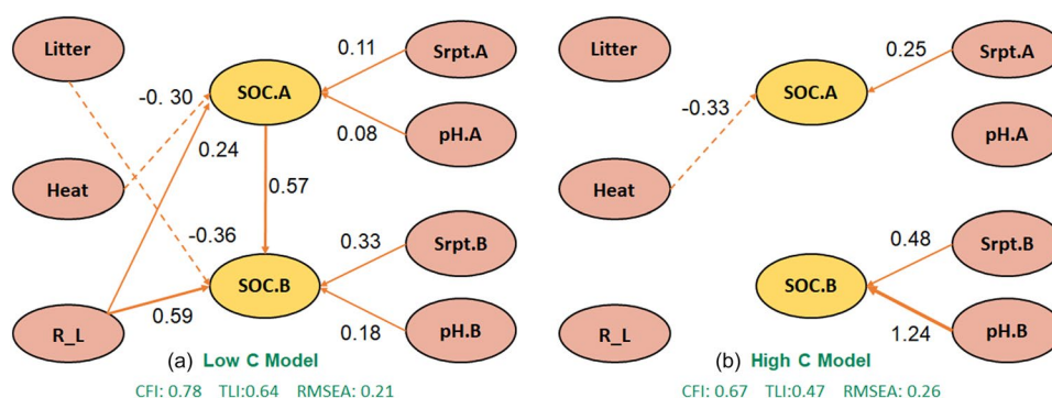
Figure 4. SEM low-SOC (a) and high-SOC (b) model of the effects of environmental (Litter, Heat, and R_L) and edaphic (Srpt.A, Srpt.B, pH.A, and pH.B) factors on topsoil and subsoil SOC variation fitted using data across NEON soil plots. Litter factor was based on multi-year average net primary production reflecting long-term land use. Heat factor was represented by five observed variables—solar radiance, potential evapotranspiration, minimum and maximum annual temperatures, and vapor pressure deficit. Precipitation, topographic position index, and segment/break numbers of land-cover and land-use change derived from CCDC (Continuous Change Detection and Classification) were used to characterize the runoff/erosion and leaching potential factor (R_L). The mineral sorption factor of topsoil (Srpt.A) and subsoil (Srpt.B) was calculated based on the ratio of clay content to cation exchange capacity for each soil layer. pH.A: pH of topsoil; pH.B: pH of subsoil. The CFI (comparative fit index), TLI (Tucker Lewis index), and RMSEA (root mean square error of approximation) are fit indices of the model.
