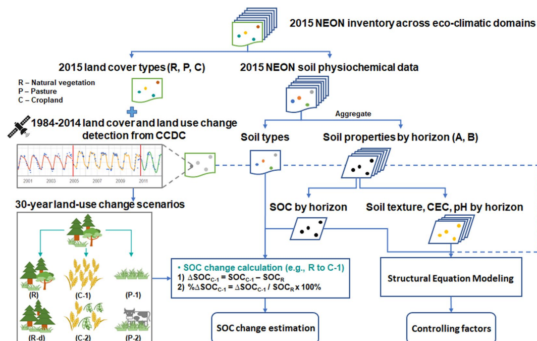
Figure 1. Flow chart of the data analysis.
