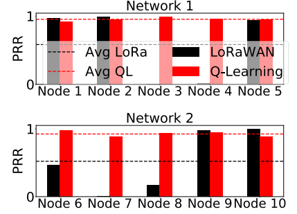
Figure 14: PRR comparison with LoRaWAN under no retransmissions
