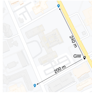
Figure 15: Outdoor deployment.
