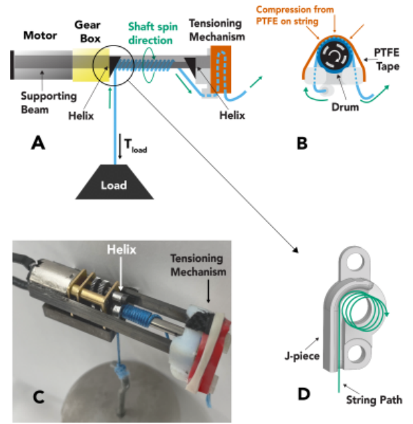
Fig. 3. A) Side view illustration of the miniature capstan winch with core components labeled. B) End view showing the tensioning mechanism. C) Isometric photo of the winch. D) CAD rendering of the helix and "J" piece.
