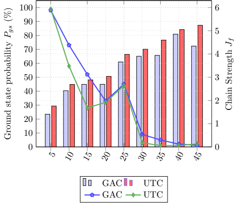
Fig. 7: Comparison between chain strengths derived from GAC and UTC. The ground state probability corresponds to each algorithm is also reported with annealing\_time = 1000 , num\_reads = 100 .
