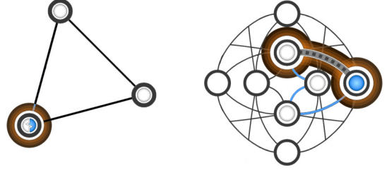
Fig. 1: A logical representation of an Ising Hamiltonian with three variables (left) is mapped onto D-Wave 2000Q-6 Chimera topology (right). A chain of qubits is connected by grey dash line. Solid blue lines represent original couplings.
