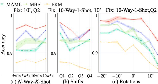
Figure 5: AffNIST results.
