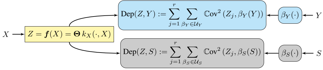
Figure 2: Our IRepL model consists of three components: i) An r -dimensional encoder f belonging to the universal RKHS \mathcal{H}_X . ii) A measure of dependence that accounts for all dependence modes between data representation Z and semantic attribute S induced by the covariance between Z = f(X) and \beta_S(S) where \beta_S belongs to a universal RKHS \mathcal{H}_S . iii) A measure of dependency between Z and the target attribute Y defined similarly as that for S .
