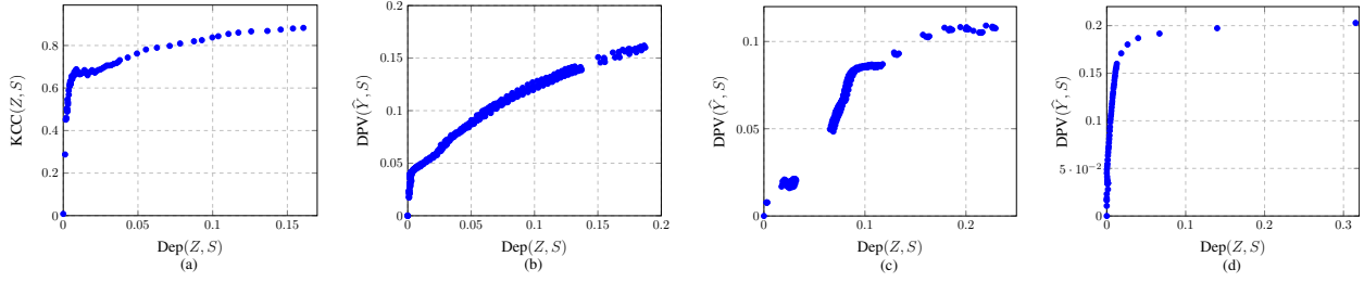
Figure 6: Invariance versus \text{Dep}(Z, S) of K-\mathcal{T}_{\text{Opt}} for (a) Gaussian, (b) Folktables-WA, (c) Folktables-NY, and (d) CelebA datasets. \text{Dep}(Z, S) enjoys a monotonic relation with the underlying invariance measures.
