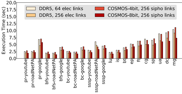
Fig. 12. Performance comparison of OPCM with DDR5.
