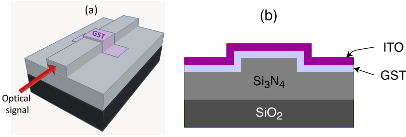
Fig. 2. (a) 3D view of GST-based PCM cell. (b) Cross-sectional view of GST deposited on a \text{Si}_3\text{N}_4 waveguide.
