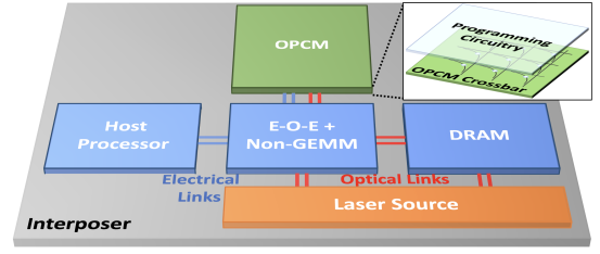
Fig. 2. Architecture of an OPCM-based computing system.
