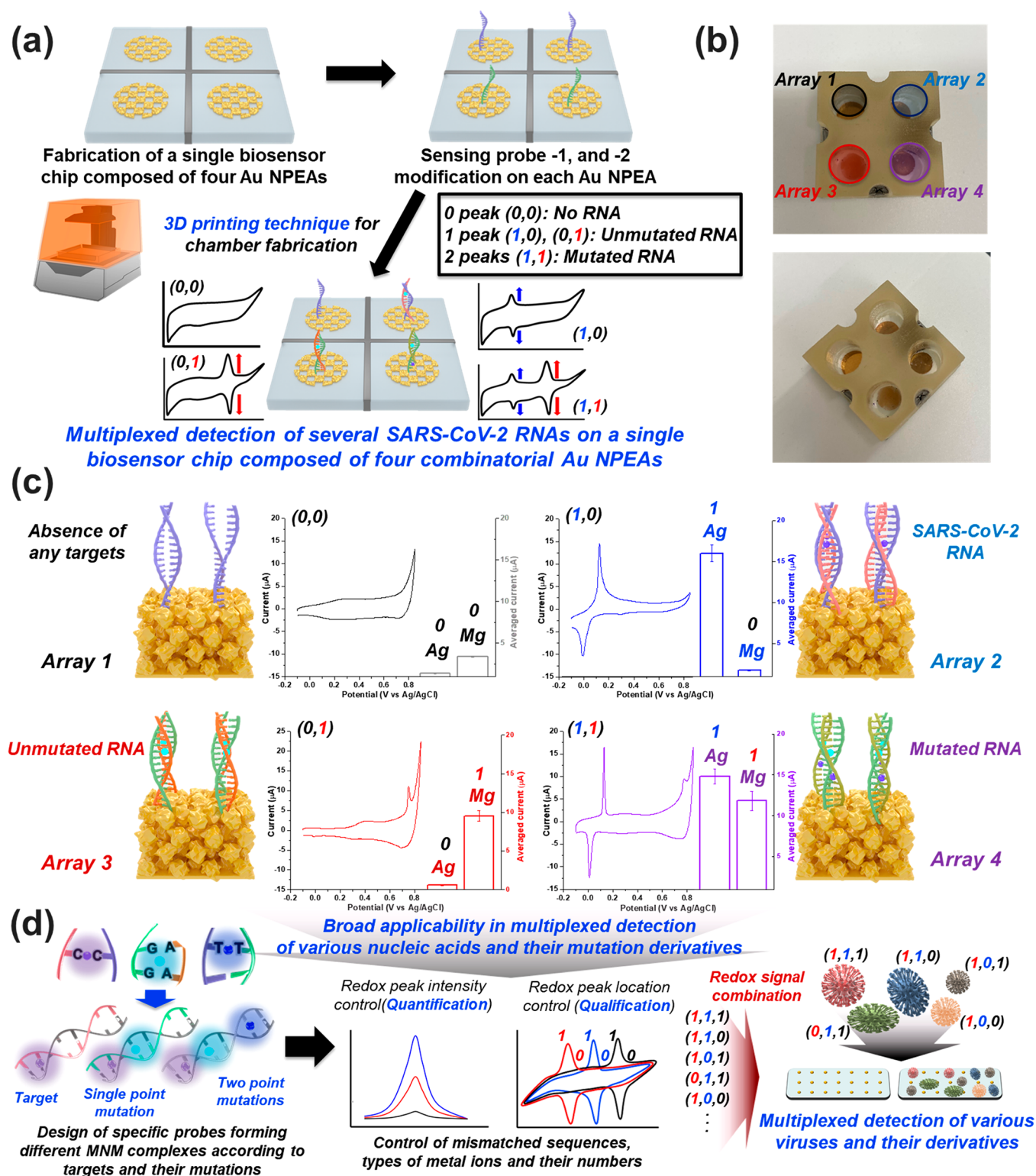
Figure 5. Multiplexed detection of several SARS-CoV-2 RNAs on the single biosensor chip composed of four combinatorial Au NPEAs. (a) Schematic image of multiplexed detection of several SARS-CoV-2 RNAs on a single biosensor chip composed of four combinatorial Au NPEAs fabricated using a 3D printing technique. (b) Optical images of a 3D-printed chamber-attached single biosensor chip. (c) Cyclic voltammograms and oxidation current peak intensities of each Au NPEA on the single biosensor chip under four different conditions. Error bars show the standard error of the mean of three measurements. (d) Scheme for broad applicability of this nanobiosensor in multiplexed detection of various nucleic acids, viral RNAs, and their mutation derivatives through control of mismatched sequences, metal ions, and numbers by designing sensing probe sequences.
