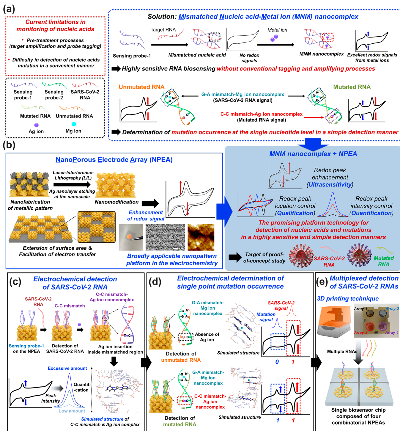
Figure 1. Electrochemical SARS-CoV-2 nanobiosensor using mismatched nucleic acid–metal ion nanocomplex on a Au NPEA. (a) Schematic diagram of nucleic acid biosensing mechanism using mismatched nucleic acids–metal ion (MNM) nanocomplex formation for highly sensitive SARS-CoV-2 RNA detection and electrochemical determination of single point mutation occurrence and its broad applicability in multiplexed detection of various nucleic acids. (b) Scheme and optical image of the Au NPEA. (c) Electrochemical detection of target single SARS-CoV-2 RNA. (d) Electrochemical determination of single point mutation occurrence in SARS-CoV-2 RNA using two different types of mismatched nucleic acids and metal ions. (e) Schematic diagram of multiplexed detection of several SARS-CoV-2 RNAs on a single biosensor chip composed of combinatorial Au NPEAs fabricated by a 3D printing technique.
