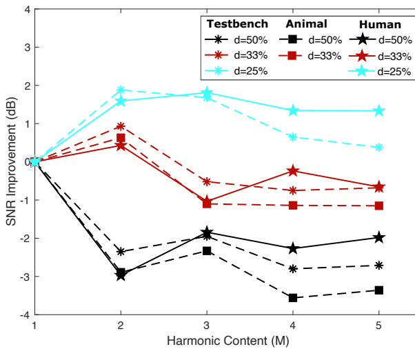
Fig. 11. SNR improvements at each \chi = (d, M) design points with respect to \chi_0 = (d, 1) .
