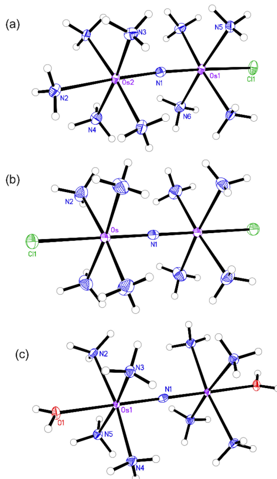
Figure 2. X-ray crystal structures of (a) compound 1 , (b) Os245, and (c) Os245'. Outer-sphere solvent molecules and counterions are omitted for clarity. Ellipsoids are drawn at the 50% probability level. For Os245', only one of the two independent molecules present in the asymmetric unit is shown. Unlabeled atoms are symmetry generated. Selected geometric parameters are given in Tables S2–S5.
