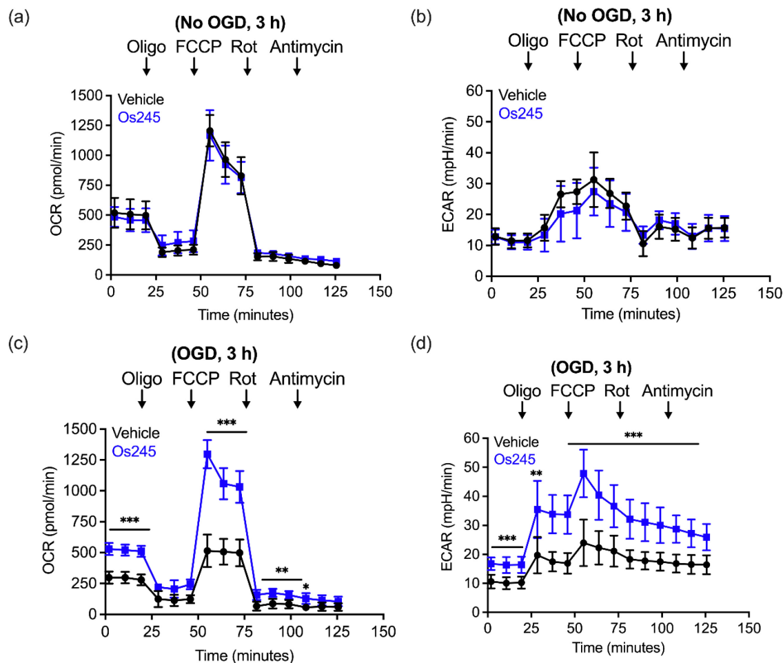
Figure 7. (a) Oxygen consumption rate (OCR) and (b) extracellular acidification rate (ECAR) measurements in primary cortical neuron cultures after the sequential addition of oligomycin (1 \mu M), FCCP (2 \mu M), rotenone (300 mM), and antimycin (1 \mu M) following treatment with Os245 (75 \mu M) for 3 h. (c,d) Pretreatment with Os245 (75 \mu M) for 3 h preserves (c) OCR and (d) ECAR in primary cortical neurons 2 h after being subjected to 30 min OGD. Data is represented as the mean \pm SD of data. * p <0.05, ** p <0.01 and *** p <0.001 as determined by two-way ANOVA followed by Bonferroni's post hoc test ( n = 3).
