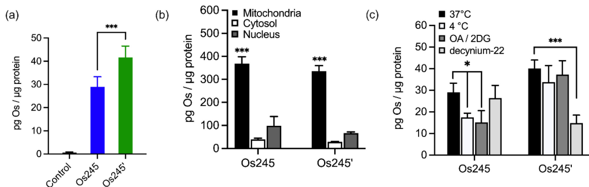
Figure 4. (a) Cellular Os accumulation in HeLa cells treated with Os245 or Os245' (50 \mu\text{M} , 3 h dose) at 37 °C. (b) Comparison of Os content in the mitochondria, cytosol, and nuclei of HeLa cells treated with Os245 or Os245' (50 \mu\text{M} , 24 h dose). (c) Cellular uptake of Os245 and Os245'
