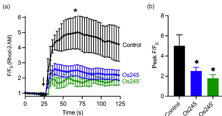
Figure 5. (a) Mitochondrial \text{Ca}^{2+} accumulation after addition of 100 \mu M histamine in HeLa cells
