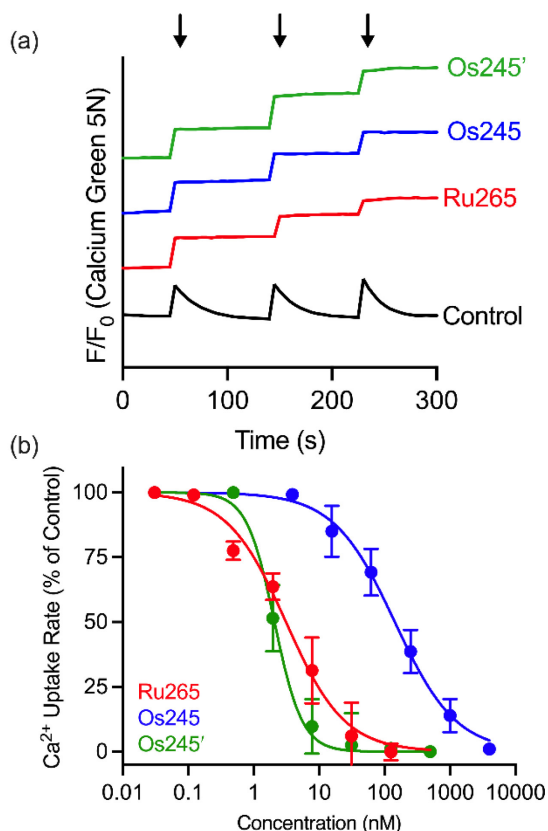
Figure 3. (a) Representative traces of extramitochondrial \text{Ca}^{2+} clearance in permeabilized HeLa cells ( 5 \times 10^6 cells \text{mL}^{-1} ) treated with 1 \mu\text{M} of Ru265, Os245 or Os245'. Arrows indicate addition of 10 \mu\text{M} \text{Ca}^{2+} . The traces are vertically offset for clarity. (b) Dose-response curve for mt- \text{Ca}^{2+} uptake inhibition by Ru265, Os245, and Os245' in permeabilized HeLa cells. Data are represented as the mean \pm SD ( n = 4-5 ).
