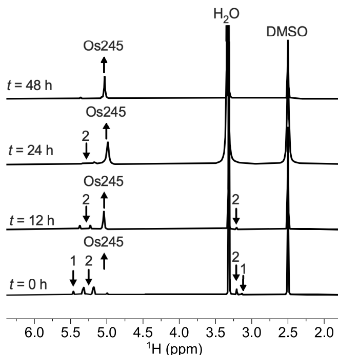
Figure 1. ^1\text{H} NMR spectra (500 MHz, 25 °C, \text{DMSO-}d_6 ) showing the conversion of 1 and 2 to Os245 by heating in refluxing HCl. Arrows indicate the growth or disappearance of peaks.
