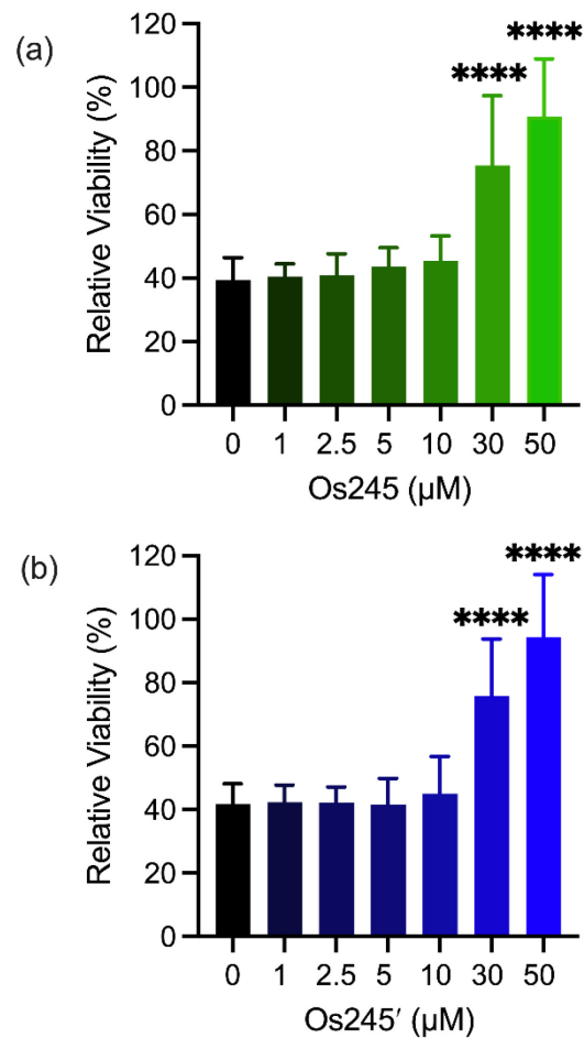
Figure 6. Cell viability in primary cortical neuron cultures treated with increasing concentrations of Os245 or Os245' for 3 h before being subjected to a lethal period of OGD (90 min). Cell viability was measured using the MTT assay 24 h after OGD. Bars represent the mean + SD. **** p < 0.0001 relative to vehicle (0 \mu\text{M} ) as determined by Mann–Whitney U tests ( n = 4 ).
