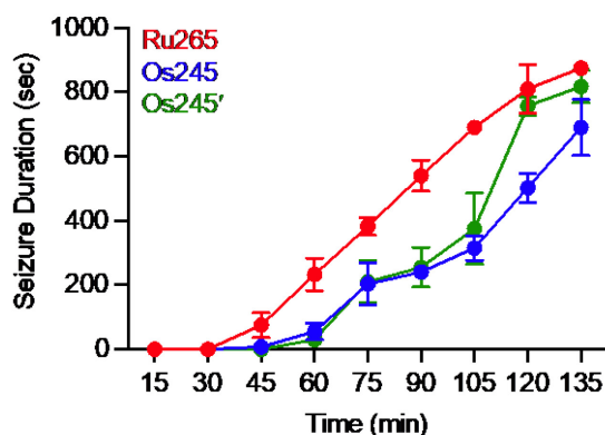
Figure 8. Seizure duration in male C57/Bl6 mice injected i.p. with 10 mg/kg of Ru265, Os245, or Os245'.
