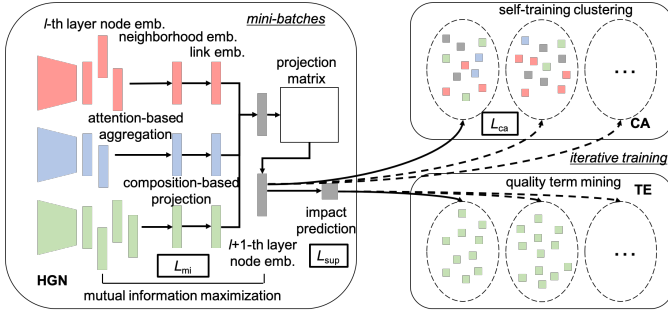
Fig. 2. The overall architecture of CATE-HGN.
