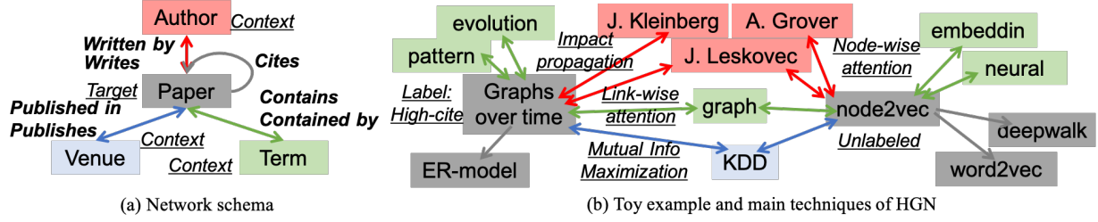
Fig. 1. The schema and toy example of real-world heterogeneous publication network.
