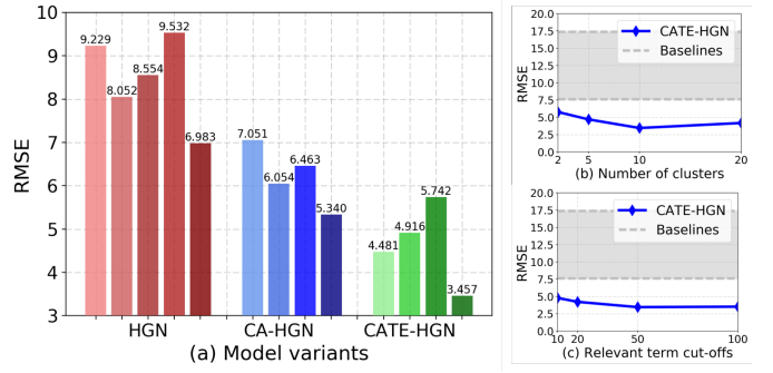
Fig. 4. In-depth study on the performance of CATE-HGN regarding the impact of model components and hyper-parameters.
