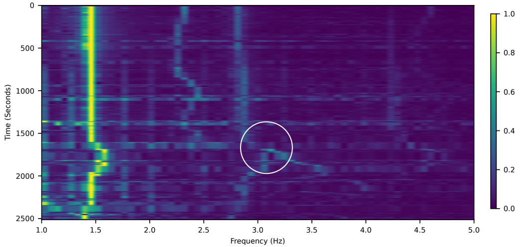
Fig. 13: The peaks of FHR &amp; MHR's 2nd harmonic crossing over each other at a certain point in time and confusing the peak tracker. This causes the tracker to follow the wrong peak after the crossover
