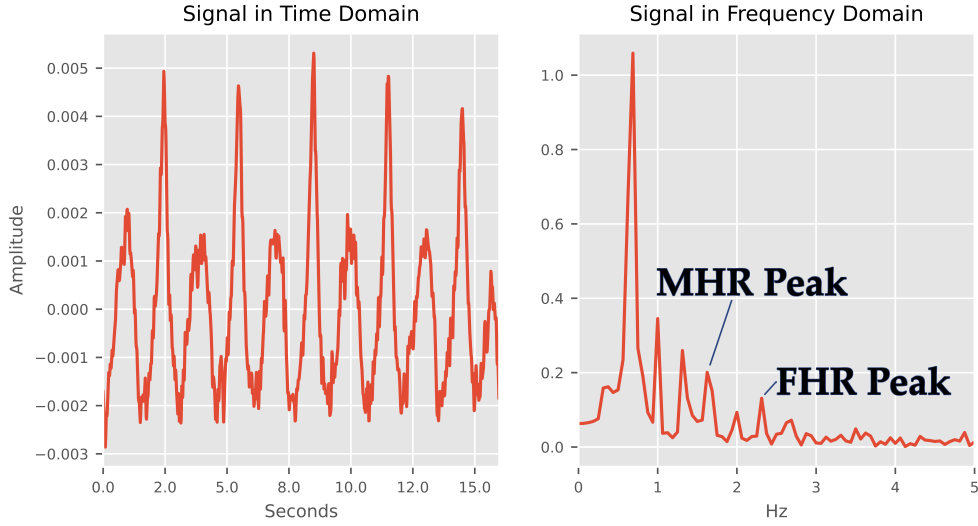
Fig. 11: An Rt-Traq wave generated using Constant Window Count, which is able to reinforce and clearly show the FHR & MHR peaks in its spectrum. A series of Rt-Traq waves generated per second allows us to trace the frequency peaks over time. This Rt-Traq wave was generated with the optimal parameters, W = 30 & L = 1280 .
