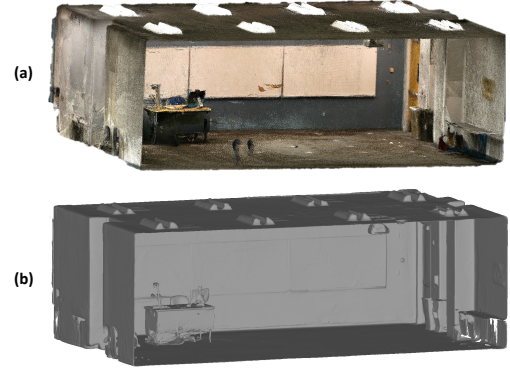
Figure 2: (a) Point cloud generated from the RGB-D images and (b) 3D reconstruction example.
