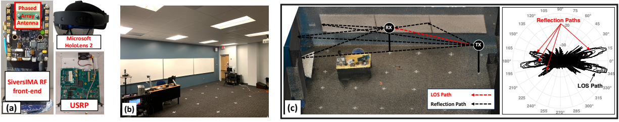
Figure 1: (a) mmWave Devices and HoloLens 2 used in the measurement, (b) measurement environment, (c) an example of collected power angular profile.
