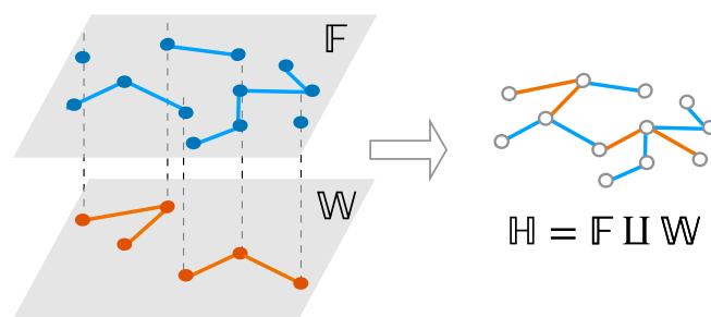
Fig. 1. Multilayer network model: An illustration of a two-layer contact network for modeling the spread of an infection over the friendship/neighborhood network \mathbb{F} and work network \mathbb{W} . The resultant contact network \mathbb{H} = \mathbb{F} \sqcup \mathbb{W} . Neighboring nodes in \mathbb{H} can transmit infections to their neighbors either through links in the \mathbb{F} network (i.e., through type f links) or \mathbb{W} network (through type w links).
