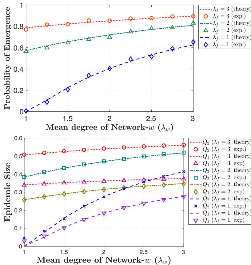
Fig. 4. Probability of emergence and the expected epidemic size for a contact network comprising two Poisson layers with mean degrees \lambda_f and \lambda_w , respectively. The fixed parameters are \tau_1^f = 0.5 , \tau_2^f = 0.7 , \tau_1^w = 0.3 , \tau_2^w = 0.4 , \mu_{11}^f = \mu_{11}^w = 0.2 , \mu_{22}^f = \mu_{22}^w = 0.5 , n = 10,000 , and we vary \lambda_f and \lambda_w in the interval [1, 3] .
