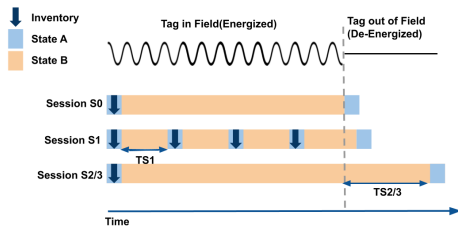
Fig. 6. Tag behaviors with different sessions
