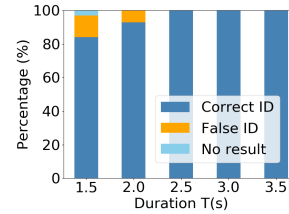
Fig. 16. Impact of signal collection time T
