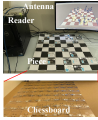
Fig. 9. Prototype environment
