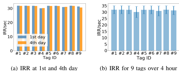
(a) IRR at 1st and 4th day (b) IRR for 9 tags over 4 hour Fig. 5. Stability performance of nine modules
