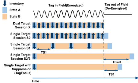
Fig. 7. Tag behaviors of different reader setups
