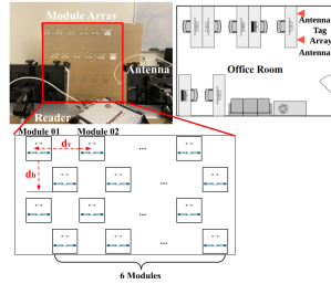
Fig. 10. Deployment of the tag array in an office
