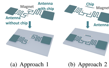
Fig. 4. Tag modification approaches
