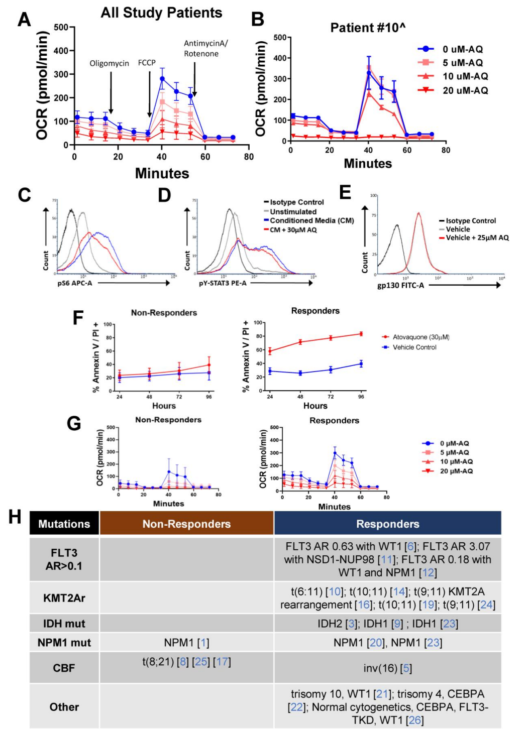
Figure 5. Atovaquone induces a dose-dependent suppression of basal and maximal mitochondrial respiration of AML primary samples, has minimal effect on pS6 and pYSTAT3, and evaluation of the OCR and cytogenetics/mutations for non responders vs. responders to ex vivo AQ. (A) Dose-dependent reductions in the oxygen consumption rate (OCR) of primary AML cells after
