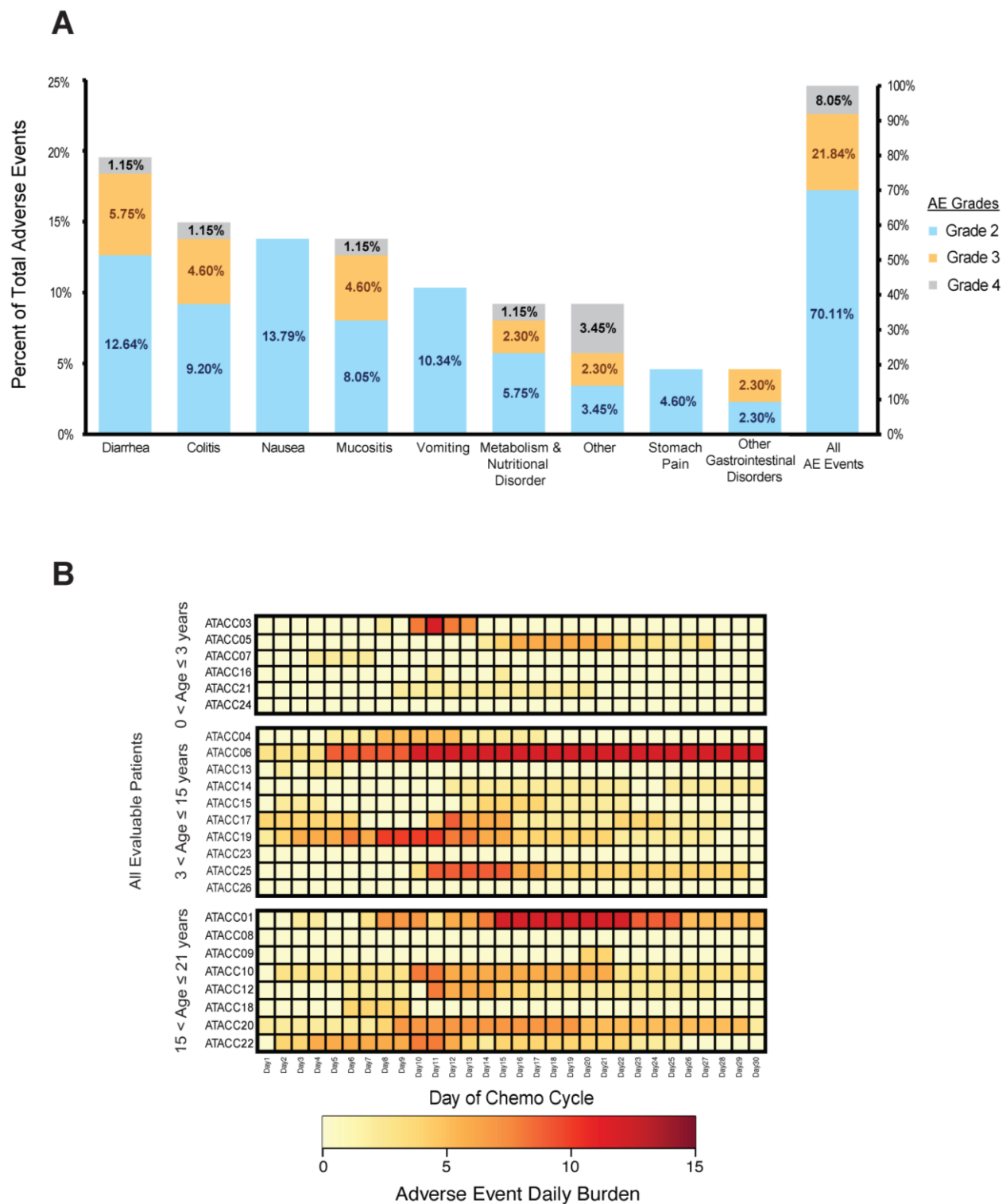
Figure 3. Gastrointestinal toxicity adverse events during atovaquone treatment. (A) Distribution of all GI-related adverse events reported on the trial. Each bar represents the percentage that each AE type was observed during the trial; small boxes represent the grades that were recorded for each AE type; percentages in the box represents the chance of an AE at a specific grade occurred during this trial. (B) Heatmap of adverse event daily burden (sum of all AE grades assigned each day) for each evaluable patients ( n = 24 ) throughout the treatment period, patients are group into their respective age ranges.
