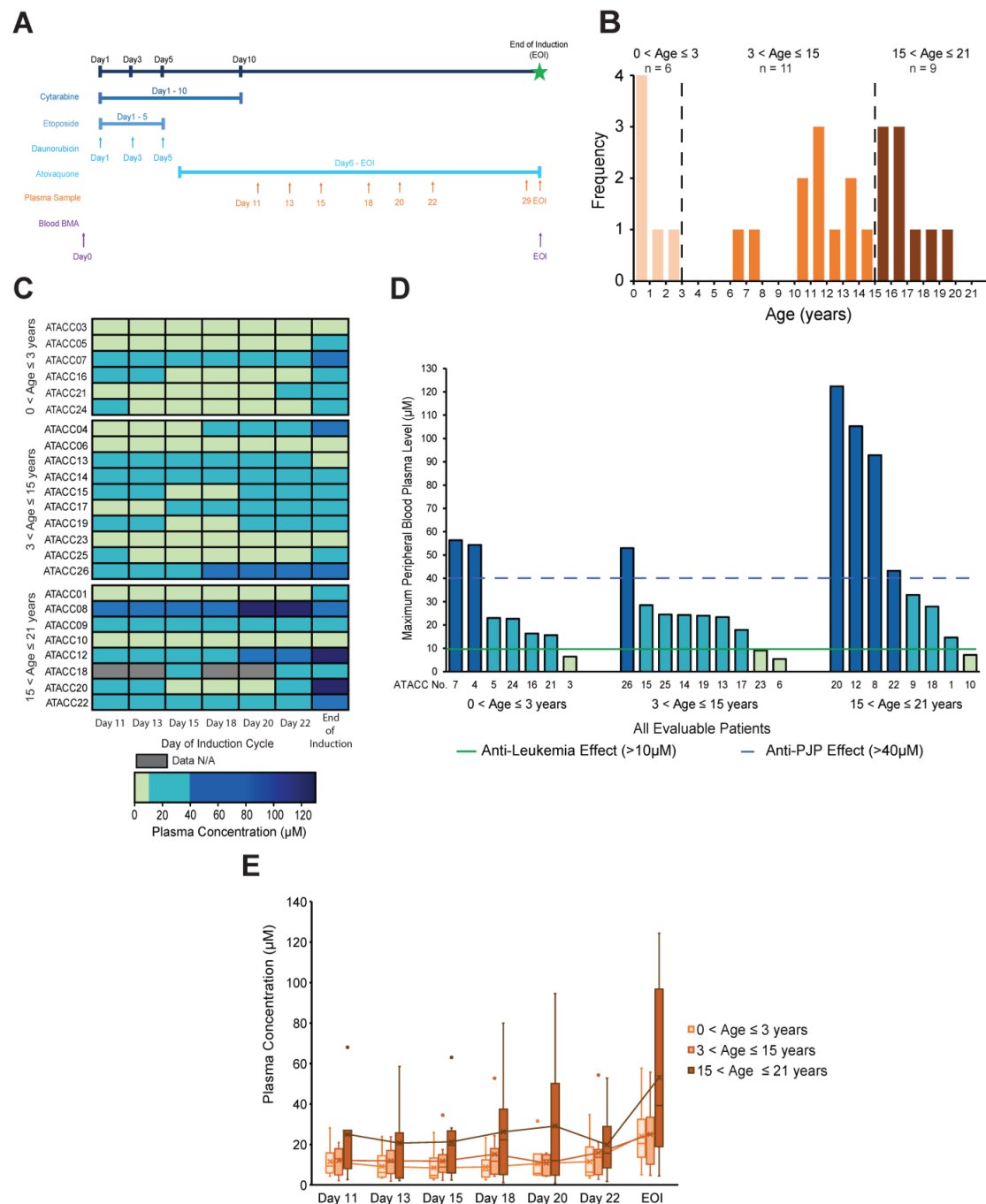
Figure 1. Plasma concentrations of atovaquone during treatment. (A) Schema of Induction 1 treatment period including administration of chemotherapy and sampling times. (B) Age distribution of patients included in the clinical trial. (C) Overview of plasma concentrations (μM) in the peripheral blood for each of the 24 patients (grouped by age range based on (B) after starting atovaquone administration. Concentrations were measured on days 11, 13, 15, 18, 20, 22, and at the end of induction (EOI). (D) Maximum peripheral blood plasma concentrations (μM) achieved for each patient. (E) Whisker plot showing the ranges and averages atovaquone peripheral blood plasma concentrations achieved within each age group. X indicates mean concentration; top and bottom vertical lines indicate maximum and minimum values, respectively; top horizontal line of the box indicates 3rd quartile, bottom horizontal line indicates 1st quartile.
