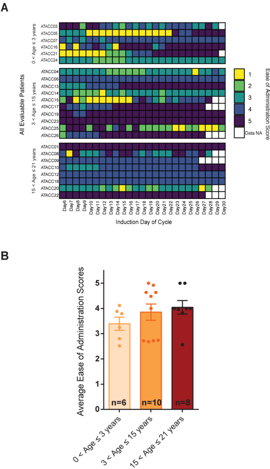
Figure 2. Distribution of ease of administration scores. (A) Overview of ease of administration score distribution during administration of atovaquone for all evaluable patients (24) on study, grouped by their age groups. Scoring scale: 1 = very difficult to administer (yellow) to 5 = very easy to administer atovaquone (dark blue). (B) Average ease of administration scores for each age group of patients (Error bars represent SEM).
