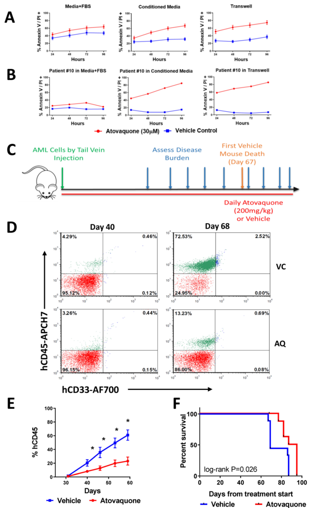
Figure 4. AQ induces apoptosis for ex vivo patient samples and Single-agent treatment with AQ decreases disease burden and prolongs survival in a patient-derived xenograft model. (A) Composite data on spontaneous vs. atovaquone induced apoptosis of primary patient samples incubated in different conditions: media with 20% fetal bovine serum (FBS), HS-5 conditioned media, or co-cultured
