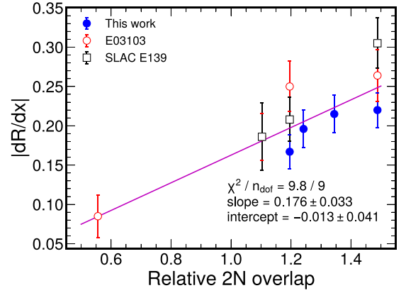
FIG. 3. Size of the EMC effect vs. relative 2N overlap, \langle O_N \rangle - \langle O_D \rangle . Data points are the same as in Fig. 2. The datum from CLAS is excluded due to inconsistencies with world data as well as possible systematic effects from the use of a different approach to radiative corrections.
