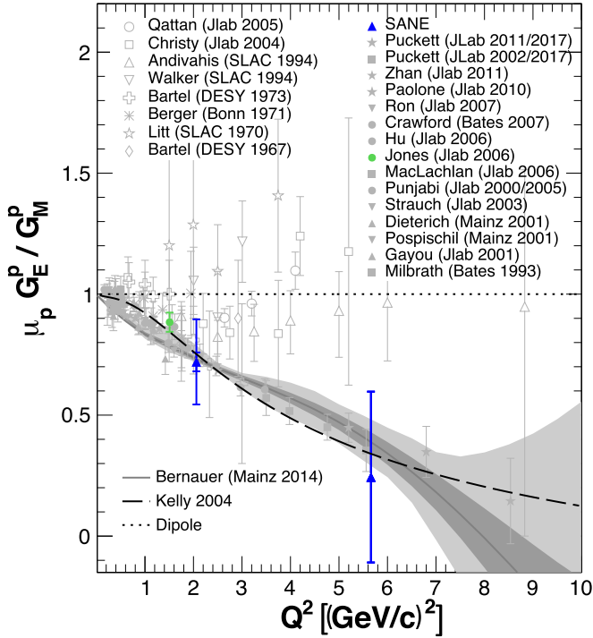
FIG. 11. The form factor measurements from SANE together with the world data as a function of Q^2 . The small error bar at the first data point at Q^2 = 2.06 is the systematic error that was explicitly studied for that point. The outer error bar is the total error bar, which is obtained by adding the statistical and systematic errors in quadrature. Since the systematic error is very small compared to the statistical error at the larger Q^2 ( Q^2 = 5.66 ), only the total error bar is shown at Q^2 = 5.66 . The previous polarized target experiment data is also highlighted (green) [32]. The gray colored error band shows the results for a global fit to form factor ratio data under the inclusion of a TPE parametrization [35]. Dark gray line: Best fit to the data. Dark gray area: Statistical 68% pointwise confidence band. Light gray area: experimental systematic error.
