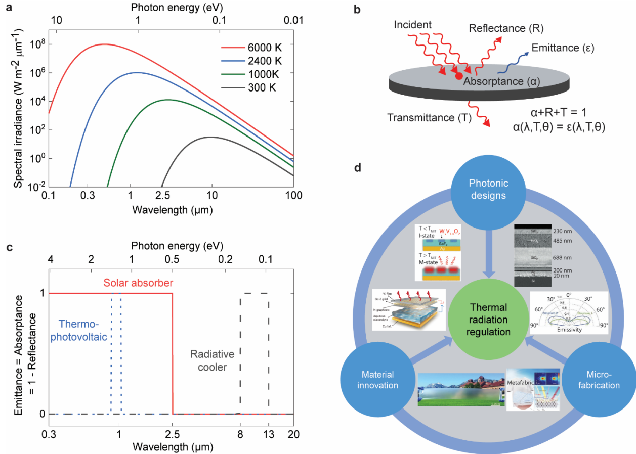
Fig. 1 (a) Radiation spectra of black bodies at different temperatures. (b) illustration of absorptance, reflectance, and transmittance. (c) Ideal spectra for opaques cases. (d) Recent key progress on innovations in fundamental photonic designs, material innovation and microfabrication [5-10].
