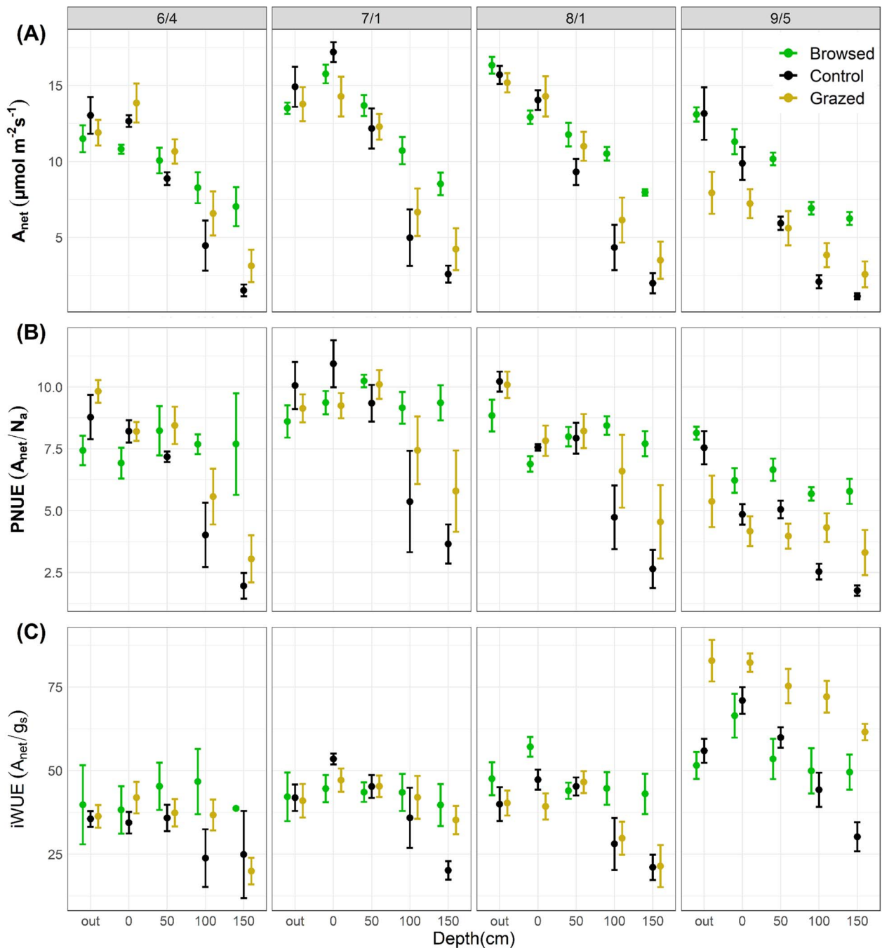
Figure 5. (A) Ambient photosynthetic rates, (B) photosynthetic nitrogen-use efficiency and (C) intrinsic water-use efficiency of leaves in C. drummondii canopies varying by canopy position (out, 0 cm, 50 cm, 100 cm and 150 cm), herbivory treatment (browsed, control and grazed) and sampling period (6/4, 7/1, 8/1, 9/5). Point and whiskers represent the mean \pm standard error.
