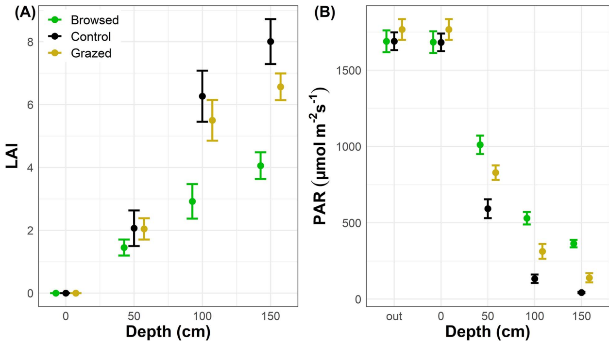
Figure 2. (A) LAI and (B) PAR measured in C. drummondii canopies at varying canopy depths (out, 0 cm, 50 cm, 100 cm and 150 cm) and herbivory treatments (browsed, control, grazed). Point and whiskers represent the mean \pm standard error of the one sampling period for LAI and the mean \pm standard error for all four sampling periods for PAR.
