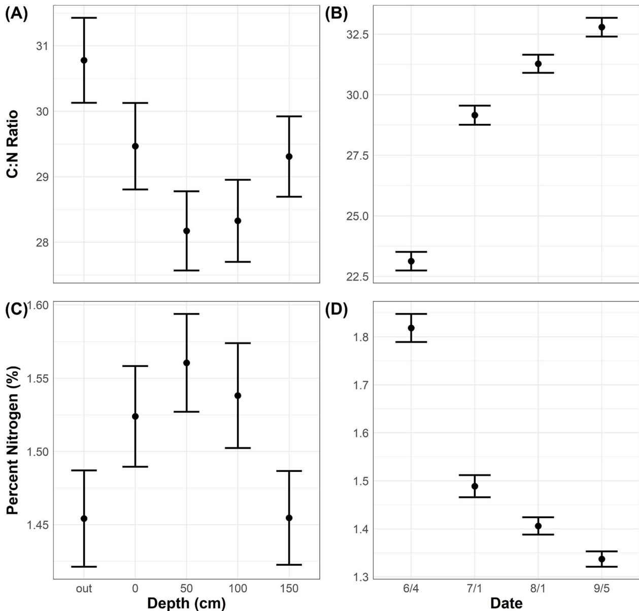
Figure 4. C:N ratio of leaves varying by depth (A) and date (B), and %N of leaves varying by depth (C) and date (D). Point and whiskers represent the mean \pm standard error.
