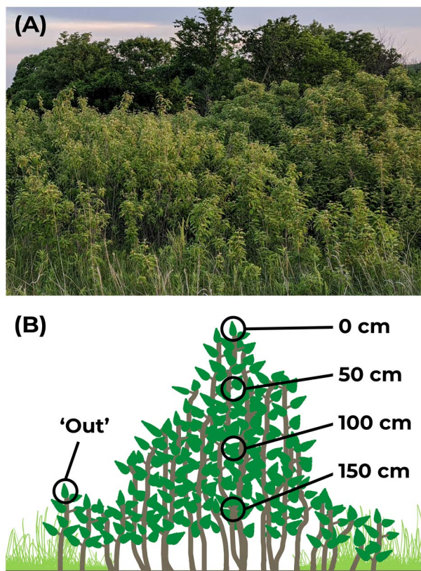
Figure 1. (A) A large island of C. drummondii with a dense canopy on watershed K4A at KPBS, Manhattan, Kansas. The growth form of C. drummondii consists of dense clonal patches of interconnected ramets termed 'islands'. (B) Diagram showing a cross section through the center of a C. drummondii island illustrating its growth form and our sampling locations. Black circles represent the measurement location for each canopy depth. Diagram credit: C. drummondii island animation by Emily Wedel.
