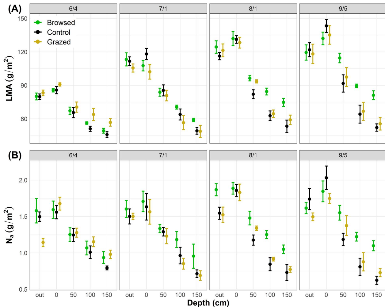
Figure 3. (A) LMA and (B) N_a of leaves in C. drummondii canopies varying by canopy position (out, 0 cm, 50 cm, 100 cm and 150 cm), herbivory treatment (browsed, control and grazed) and sampling period (6/4, 7/1, 8/1, 9/5). Point and whiskers represent the mean \pm standard error.
