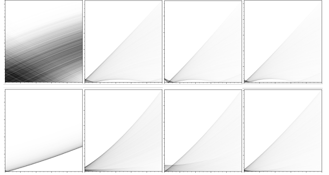
Figure 7: Complete-information auction strategies at epochs 0, 30, 60, and 90 (left to right). X and Y axes denote observation and bid, respectively. Each histogram uses 10^4 action samples per observation.
