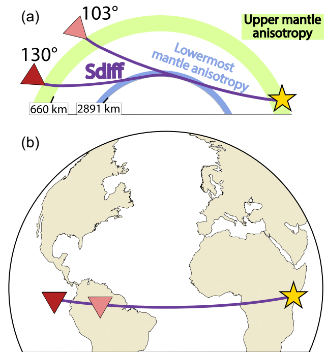
Figure 1. Schematic illustration of a typical source–receiver configuration in our numerical simulations. The S_{\text{diff}} ray path is shown by a solid purple line. (a) Cross-section through Earth. Stations are represented as red triangles and the source as a yellow star. S_{\text{diff}} potentially travels through upper mantle anisotropy at source and receiver side (green), and lowermost mantle anisotropy (blue). (b) Map view of the source, located at the equator (at longitude -90^\circ ), and the S_{\text{diff}} ray path to stations located in a distance of 103^\circ and 130^\circ at the equator.
