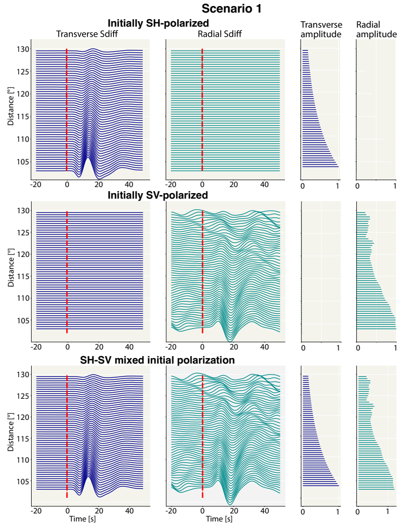
Figure 3. Displacement synthetic seismograms for simulations using PREM (Dziewonski & Anderson 1981) as an input model (scenario 1 in Fig. 2), calculated for a focal depth of 0 km. We show transverse (first column, dark blue) and radial (second column, teal) S_{\text{diff}} waveforms and corresponding transverse (third column, dark blue) and radial (fourth column, teal) amplitudes as a function of epicentral distance. The amplitudes are plotted relative to the transverse (row 1 and 3) and radial S_{\text{diff}} (row 2) amplitudes at the lowest distance and measured as the maximum absolute values in a time window of from the predicted S_{\text{diff}} arrival to 30 s after it. Three simulations are shown for SH (top row), SV (middle row) and mixed SH–SV initial polarizations (bottom row). Seismograms are shown from 20 s before the predicted S_{\text{diff}} arrival time until 60 s after. Predicted arrival times are calculated using TauP (Crotwell et al. 1999) for the PREM model (red dashed lines). Waveforms are shown after applying a 10–50 s bandpass filter.
