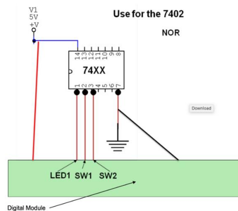
Figure 5b: Connections
