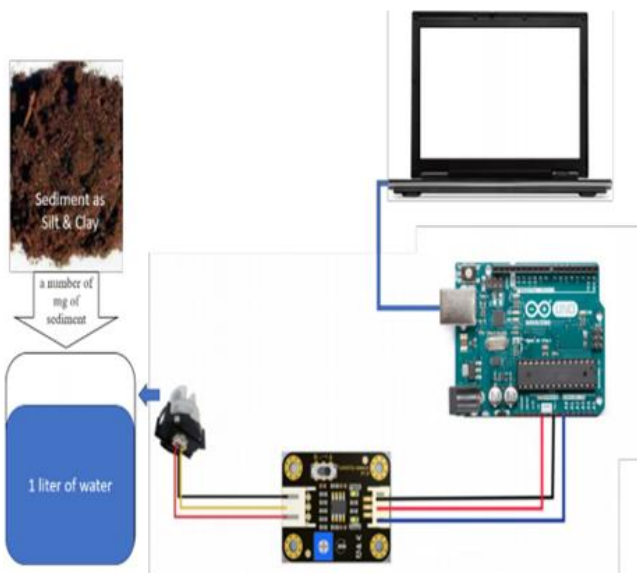
Figure 6 Experimental setup
