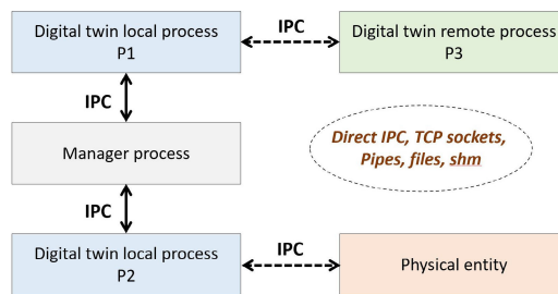
FIGURE 7. Inter-process communication (IPC) among digital twin processes.
