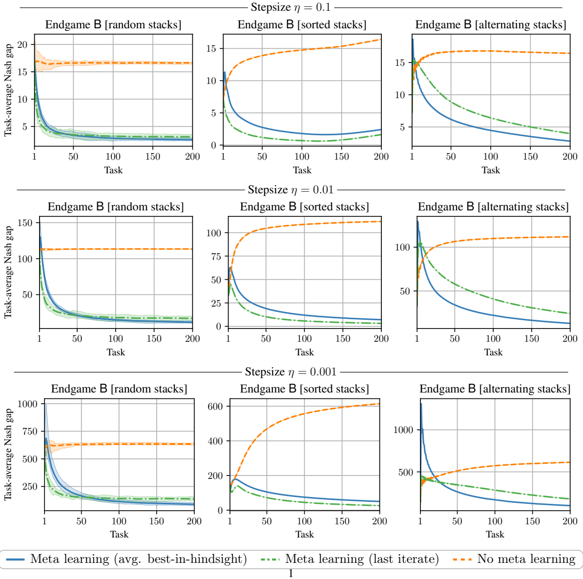
Figure 3: Vanilla OGD versus our meta-learning versions of OGD for different values of the learning rate \eta in Endgame B.
