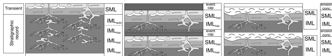
FIGURE 13. We suspect that the downcore increase in time averaging from the surface well-mixed layer (SML) to the subsurface incompletely mixed layer (IML) that is frequently observed in cores from modern environments—both these from the southern California shelf and from marine environments elsewhere (Kosnik et al. 2013; Olszewski and Kaufman 2015)—and as also predicted here by our forward models will typically not be preserved in the older, permanent stratigraphic record, at least under (A) a regime of relatively continuous, background sedimentation. Under those common conditions, deeper burrows crosscut earlier shallow-burrowing tiers as the sediment–water interface moves upward under aggradation, erasing the signature of the SML (analogous to the erasure of the uppermost segments of burrows). The strong dominance of age-frequency distributions (AFDs) by young shells typical of SMLs—that is, the left edge of the L-shaped distribution—will be lost. The AFDs of historic layers encountered in deep-time records will instead be more analogous to the less-skewed and more platykurtic (flatter) AFDs that characterize subsurface (IML) increments of Holocene cores. Exceptionally, a downcore increase in time averaging can be preserved in records from settings where (B) anoxic conditions are coupled with deposition, so that laminated sediments cap and protect the former SML from subsequent bioturbation (e.g., Savrda and Bottjer 1989) and (C) storm or turbiditic deposition does not fully erode the SML and, for one or more reasons, is not bioturbated by later colonizers (e.g., Bentley and Nittrouer 1999). Shells from the capping storm deposit might be more or less time averaged, depending on the source of those shells.
