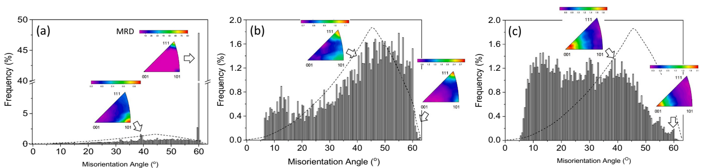
Fig. 2. Misorientation angle distribution along with the distribution of axes at rotation angle of 60^\circ and 39^\circ in a standard stereographic triangle for Ni–30Fe alloy subjected to different processing routes: a) iterative recrystallisation, b) mould casting and c) columnar casting. The dash line represents the random distribution.
