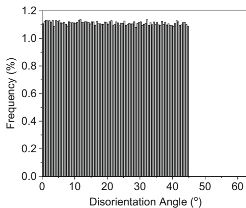
Fig. 5. The disorientation angle distribution resulted from impingement of each of pair of 1000 orientations arbitrarily selected along the \theta -fibre, ignoring sample symmetry (i.e., \phi_1 = 0-360^\circ , \phi_2 = 0-45^\circ ).
