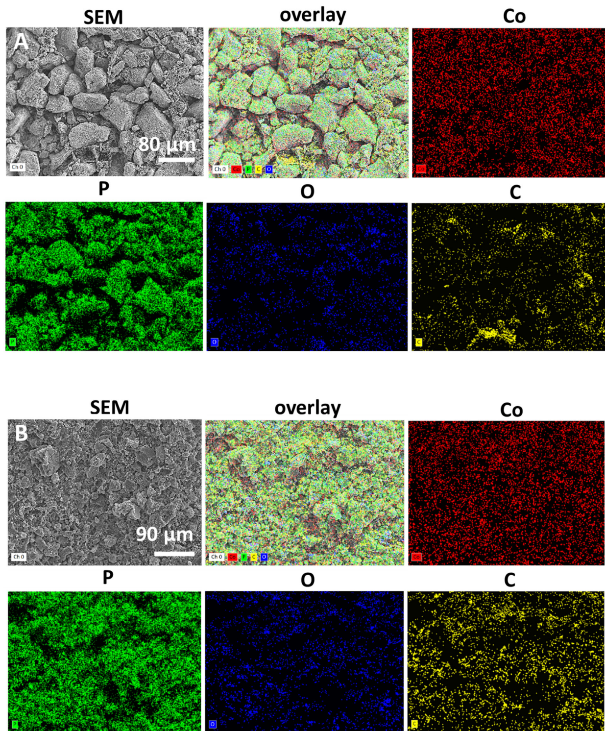
Figure S23. EDS maps of (A) \text{CoP}_3 and (B) 25\text{-CoP}_3/\text{C} embedded on \text{C}_{\text{wax}} electrode tips after 18-hour CA HER experiments.
