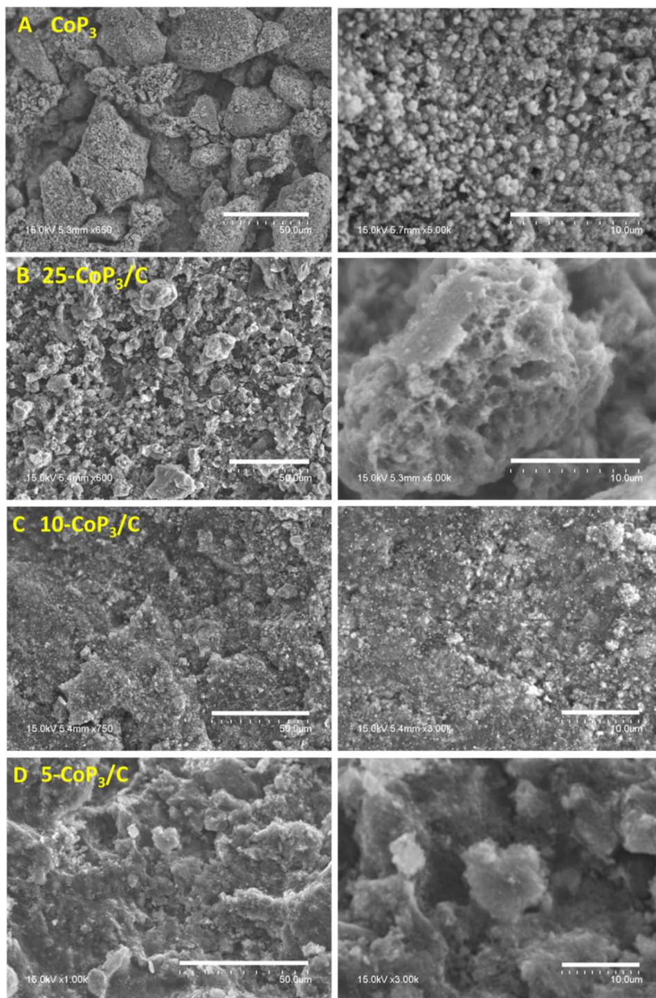
Figure S22. Scanning electron microscopy (SEM) images of (A) \text{CoP}_3 , (B) 25\text{-CoP}_3/\text{C} , (C) 10\text{-CoP}_3/\text{C} , and (D) 5\text{-CoP}_3/\text{C} embedded on a \text{C}_{\text{wax}} electrode tip after 18-hour CA HER experiments.
