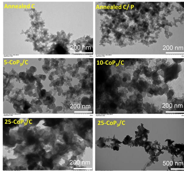
Figure 5. Representative TEM images of x-CoP 3 /C (x = 5, 10, 25 mol%) particles and aggregates synthesized from direct reactions of x-CoCl 2 /C (x = 5, 10, 25 mol%) with elemental red phosphorus at 500 °C.
