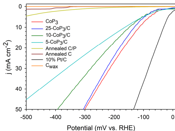
Figure 6. Representative LSV data for x -CoP 3 /C ( x = 5, 10, 25 mol%) powders on C wax electrodes using Pt counter and SCE reference electrodes in 0.5 M H 2 SO 4 (5 mV/s scan rate, no iR compensation) in a three-electrode cell. An LSV overlay graph with 85% iR compensated data is shown in Figure S15 . Plots for C wax , annealed C, annealed C/P and commercial 10% Pt/C are shown for comparison.
