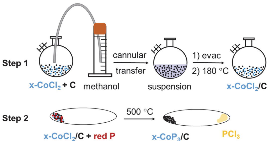
Figure 1. Schematic of two-step synthesis procedure of x- \text{CoP}_3/\text{C} ( x = 5, 10, 25 \text{ mol\%} ) materials. Step 1 shows methanol precipitation of \text{CoCl}_2 onto C (XC-72 carbon black), and step 2 shows direct reaction of x- \text{CoCl}_2/\text{C} with elemental red phosphorus at 500 °C.
