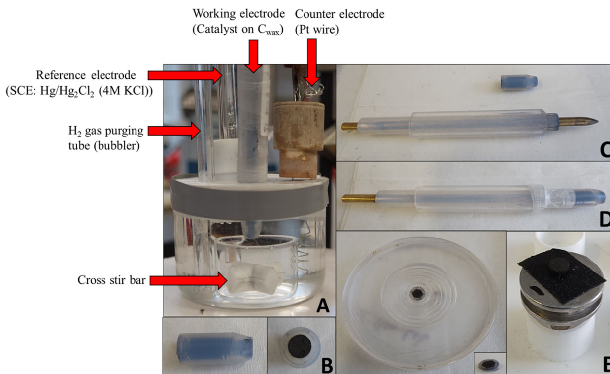
Figure S1. Images of electrochemical cell and working electrode: (A) Three electrode, single compartment cell, (B) coned, C_{wax} electrode tip in different geometries, (C) disassembled C_{wax} electrode tip + brass current collector, (D) assembled C_{wax} working electrode, and (E) cut slice C_{wax} tip geometries for post electrochemical XRD and SEM-EDS analysis.
