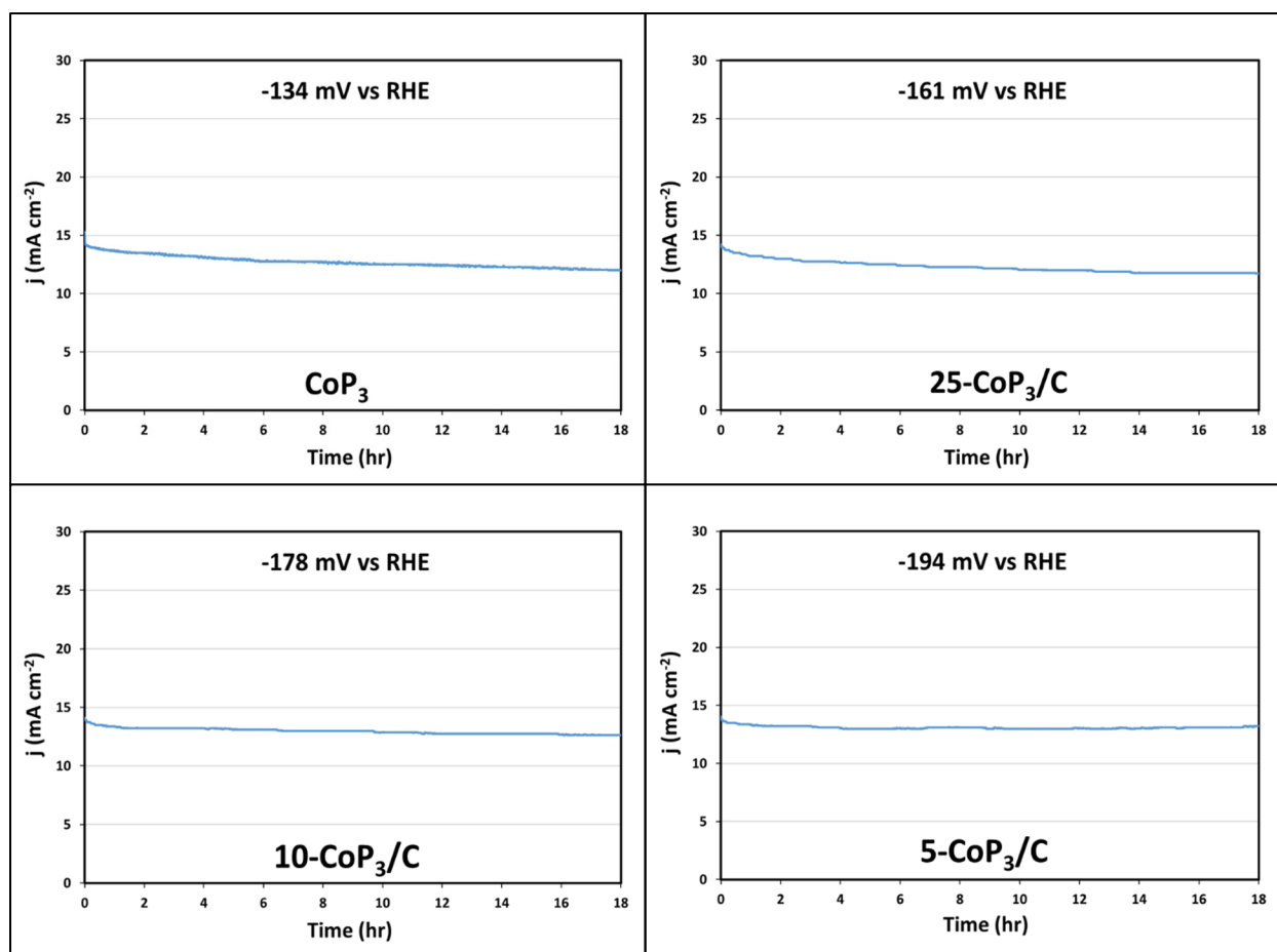
Figure S19. 18-hour constant potential chronoamperometry (CA) HER experiments for \text{CoP}_3 and x\text{-CoP}_3/\text{C} ( x = 5, 10, 25 ) catalysts using graphite rod counter electrode.
