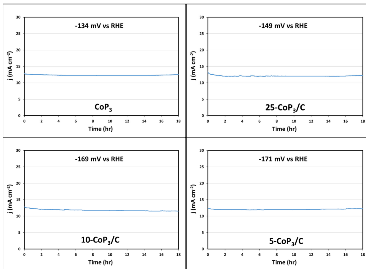
Figure S18. 18-hour constant potential chronoamperometry (CA) HER experiments for \text{CoP}_3 and x\text{-CoP}_3/\text{C} ( x = 5, 10, 25 ) catalysts using a platinum counter electrode.
