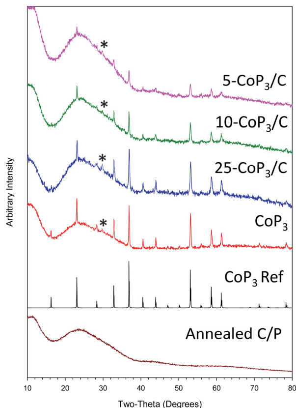
Figure 2. Powder XRD results for x\text{-CoP}_3/\text{C} ( x = 5, 10, 25 mol%) products from two-step synthesis procedure of methanol precipitations of x\text{-CoCl}_2/\text{C} ( x = 5, 10, 25 mol%) followed by direct reactions of x\text{-CoCl}_2/\text{C} with elemental red phosphorus at 500^\circ\text{C} . Reference (Ref) pattern for \text{CoP}_3 and XC-72 carbon black annealed at 500^\circ\text{C} with elemental red phosphorus are also shown. Trace \text{CoP}_2\text{O}_6 impurity are identified with a (*).
