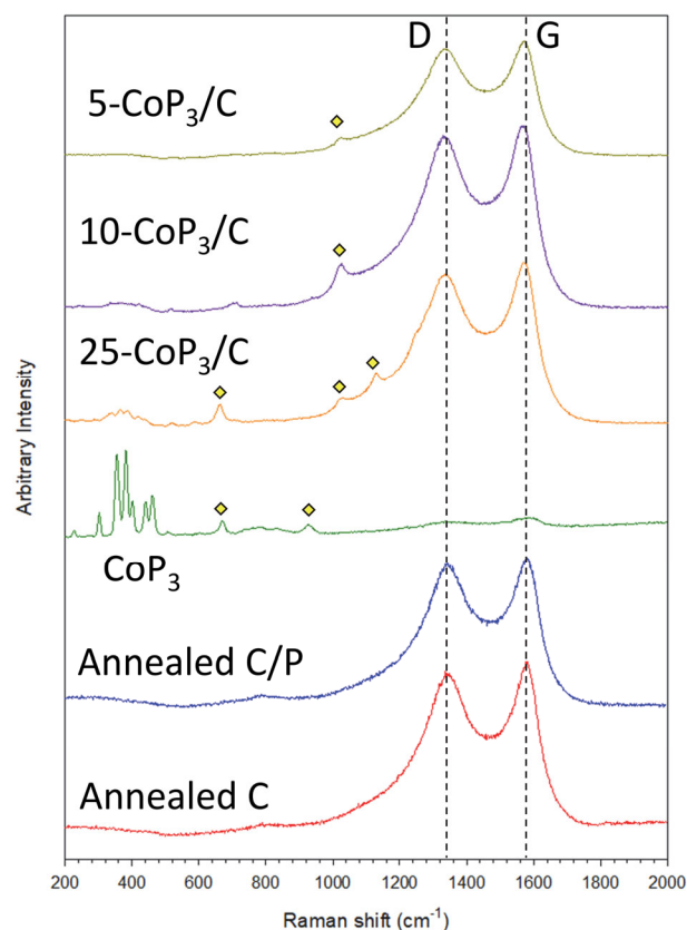
Figure 3. An overlay of Raman spectra of \text{CoP}_3 , x\text{-CoP}_3/\text{C} ( x = 5, 10, 25 ) and 500^\circ\text{C} annealed carbon black alone (C) and carbon black annealed with phosphorus (C/P) in the region of 200\text{-}2000\text{ cm}^{-1} . (◆ denotes peaks for P-O bonding).
