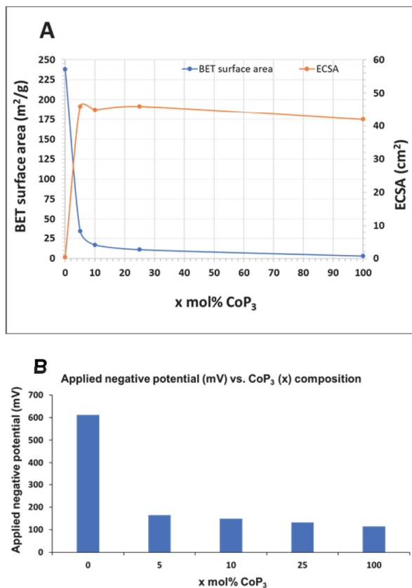
Figure 7. (A) Comparison of trends of physical BET surface area and electrochemically active surface area (ECSA) for \text{CoP}_3 and x\text{-CoP}_3/\text{C} ( x = 5, 10, 25 mol%) materials along with annealed \text{C}/\text{P} ( x=0 ). (B) variation of applied negative potentials ( iR uncompensated) to achieve a 10 \text{ mA}/\text{cm}^2 current density with the amount of \text{CoP}_3 dispersed on carbon black composites.
