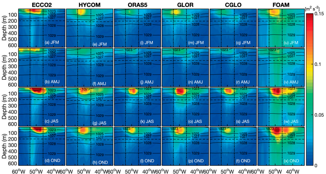
FIG. 8. Vertical structure of EKE ( \text{m}^2 \text{s}^{-2} ) and density (black contour; \text{kg m}^{-3} ) following the line in Fig. 6a. (a)–(d) ECCO2, (e)–(h) HYCOM, (i)–(l) ORAS5, (m)–(p) GLOR, (q)–(t) CGLO, and (u)–(x) FOAM. Black dashed lines mark 200-m depth. The NCB and the NCB East and West are separated by two vertical lines.
