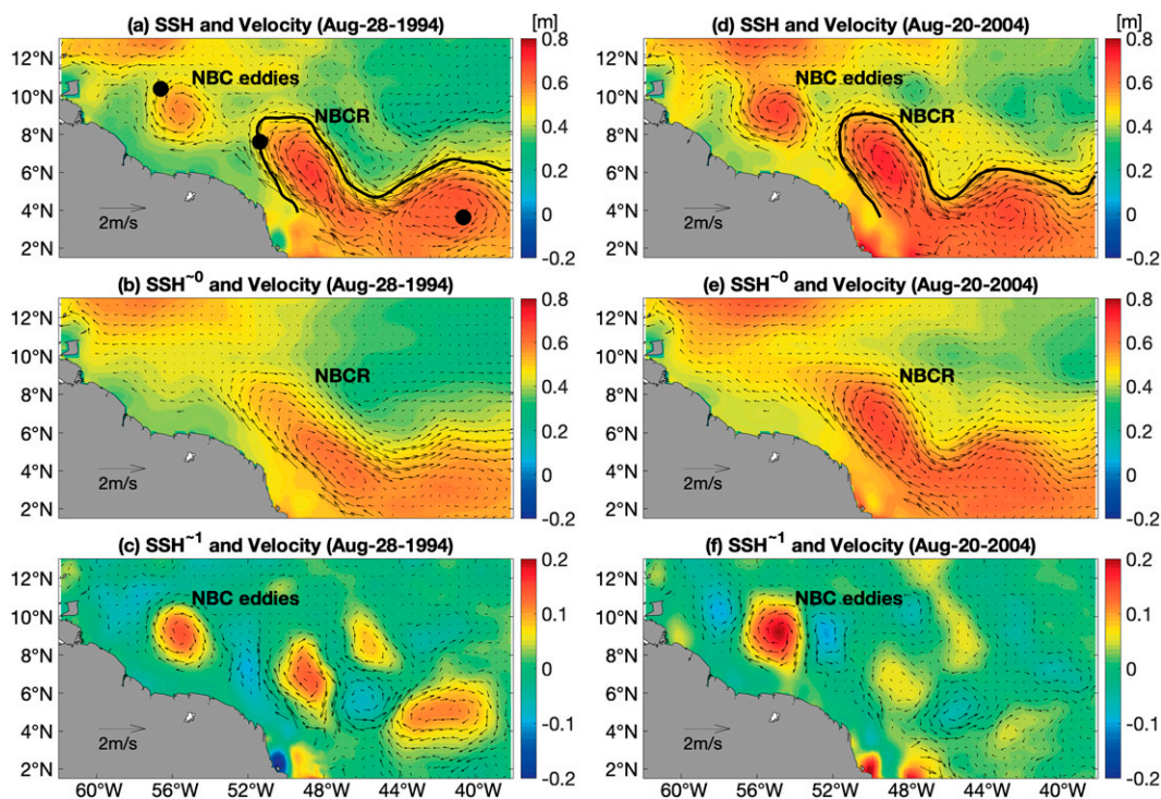
FIG. 3. Altimetry sea surface height (SSH) and geostrophic current on (left) 28 Aug 1994 and (right) 20 Aug 2004: (a),(d) original SSH field; (b),(e) MWT low-pass-filtered components (mean current); (c),(f) MWT high-pass-filtered components (eddies). The black lines in (a) and (d) (the 0.46-, 0.51-m SSH contours) mark the position of the NBC retroflection. The three black dots are used to generate Fig. 2.
