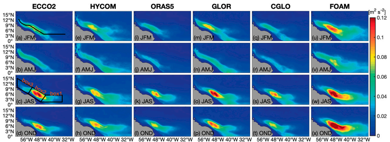
FIG. 6. Seasonal maps of the depth-mean (upper 200-m depth) EKE ( m^2 s^{-2} ). (a)–(d) ECCO2, (e)–(h) HYCOM, (i)–(l) ORAS5, (m)–(p) GLOR, (q)–(t) CGLO, and (u)–(x) FOAM. Box 2 marks the most energetic NBCR region. Box 1 and box 3 represent the NBCR East and West, respectively. The black line in (a) is used to generate Fig. 8.
