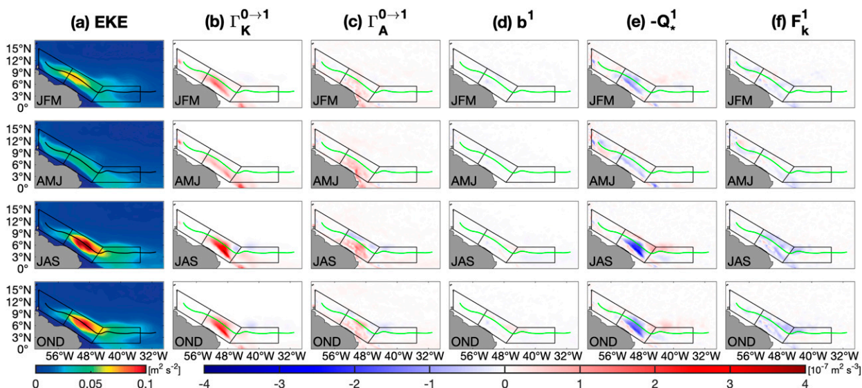
FIG. 9. Seasonal maps of the depth-mean (upper 200 m) EKE and EKE budget terms ( \text{m}^2 \text{s}^{-3} ). (a) EKE, (b) barotropic transfer from mean flow to mesoscale eddy window ( \Gamma_k^{0 \rightarrow 1} ), (c) baroclinic transfer from A^0 to A^1 ( \Gamma_A^{0 \rightarrow 1} ), (d) buoyancy conversion rate ( b^1 ), (e) nonlocal processes ( -Q_*^1 ), and (f) dissipation F_k^1 . The three boxes in Fig. 6a are shown. The black lines in (a) and green lines in (b)–(e) represent the mean eddy trajectory of all the products.
