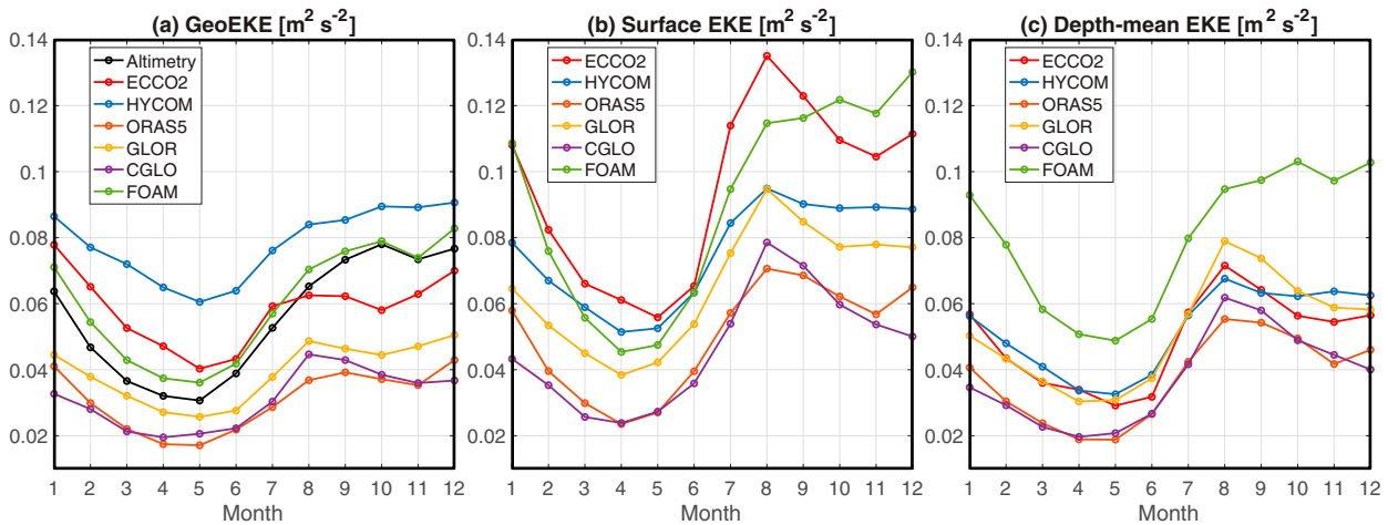
FIG. 5. Seasonal cycle of the area-mean EKE ( m^2 s^{-2} ) from (a) altimetry and six ocean reanalysis products. (b) EKE of the top layer of the six ocean reanalysis products. (c) As in (b), but for the depth-mean EKE (upper 200 m).
