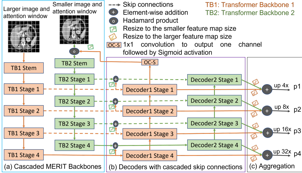
Figure 1: Cascaded MERIT architecture. (a) Cascaded MERIT backbone, (b) Decoders with cascaded skip connections from the decoder 1, (c) Prediction maps aggregation of two decoders. p1 , p2 , p3 , and p4 are the aggregated multi-stage prediction maps.
