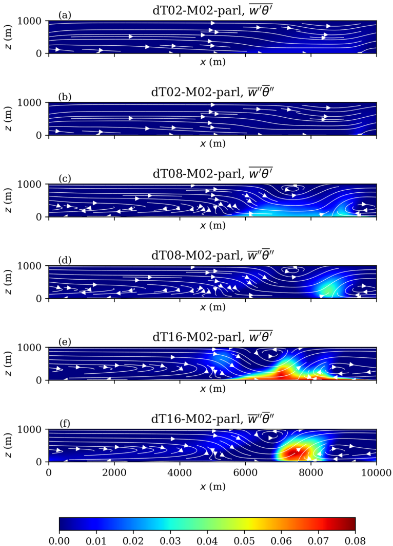
Fig. 11 Turbulent ( \overline{w'\theta'} ) and dispersive ( \overline{w''\theta''} ) heat flux ( \text{K m s}^{-1} ) overlaid with (u, w) streamlines for dT02-M02-parl, dT08-M02-parl, and dT16-M02-parl. Geostrophic wind flows into the page. All variables with an overbar are Reynolds-averaged in time and the y direction (as there is no heterogeneity in the y -direction, see Fig. 5). Ice surface is on the left half of the plot, with water surface on the right half
