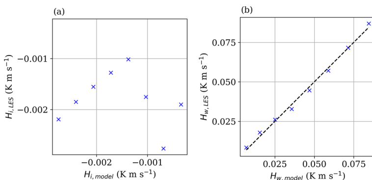
Fig. 6 a Plot of modelled versus LES heat flux spatially-averaged over the ice surface, as in Eq. 19, for the parallel cases of Suite II (all cases have an M_g = 2 \text{ m s}^{-1} ). Here, m_{parl} = -1.41 \times 10^{-4} and n_{parl}/m_{parl} = 0 . b as in a , but for the water surface, following Eq. 20, where p_{parl} = 2.96 \times 10^{-3} and q_{parl}/p_{parl} = 0.1
