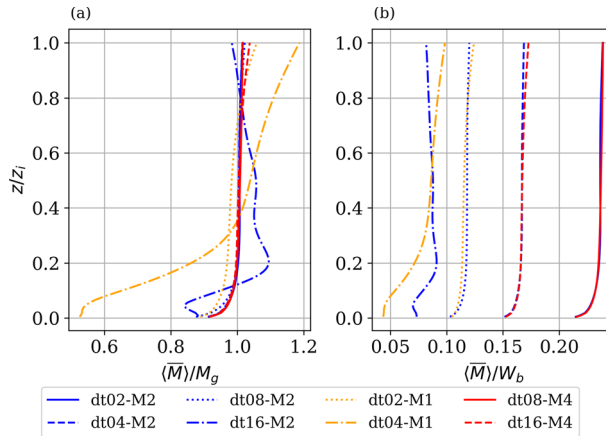
Fig. 2 a Profiles of \overline{M} , normalized by the geostrophic speed M_g . Similar line styles correspond to similar values of Ri_h . Similar line colours correspond to equal geostrophic wind speeds. b as in a , but the profiles are scaled by W_b
