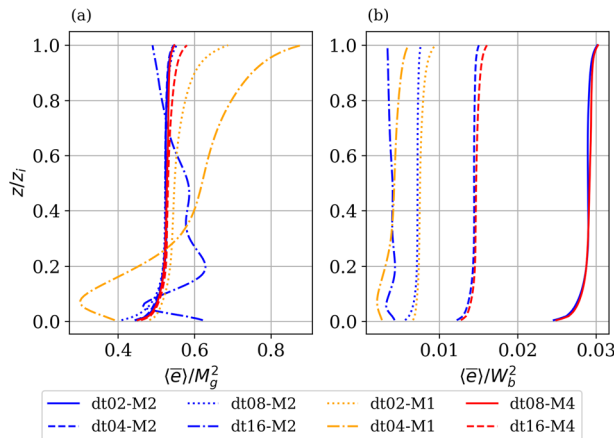
Fig. 3 a Profiles of averaged TKE, \overline{e} , normalized by the square of geostrophic speed M_g^2 . Similar line styles correspond to similar values of Ri_h . Similar line colours correspond to the equivalent geostrophic wind speeds. b as in a , but the profiles are scaled by W_b^2
