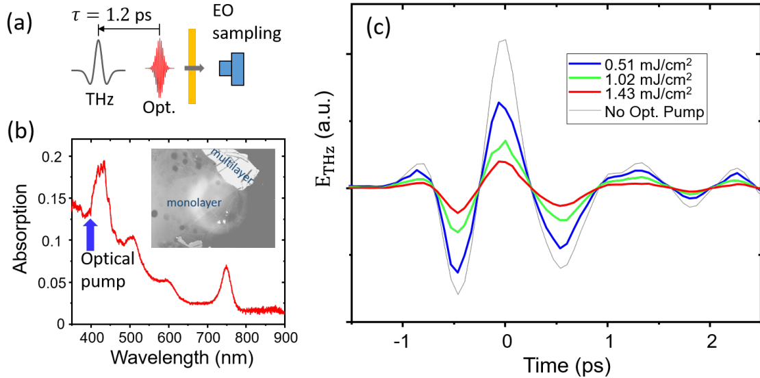
FIG. 1. (a) Schematics of the optical pump/THz probe setup (b) Optical absorption spectrum of the WSe 2 sample. A microscopic image of the sample is shown in inset. (c) THz waveforms transmitted through the sample for the optical pump fluence 0.51, 1.02 and 1.43 mJ/cm 2 . The gray line presents the waveform of no optical excitation.
