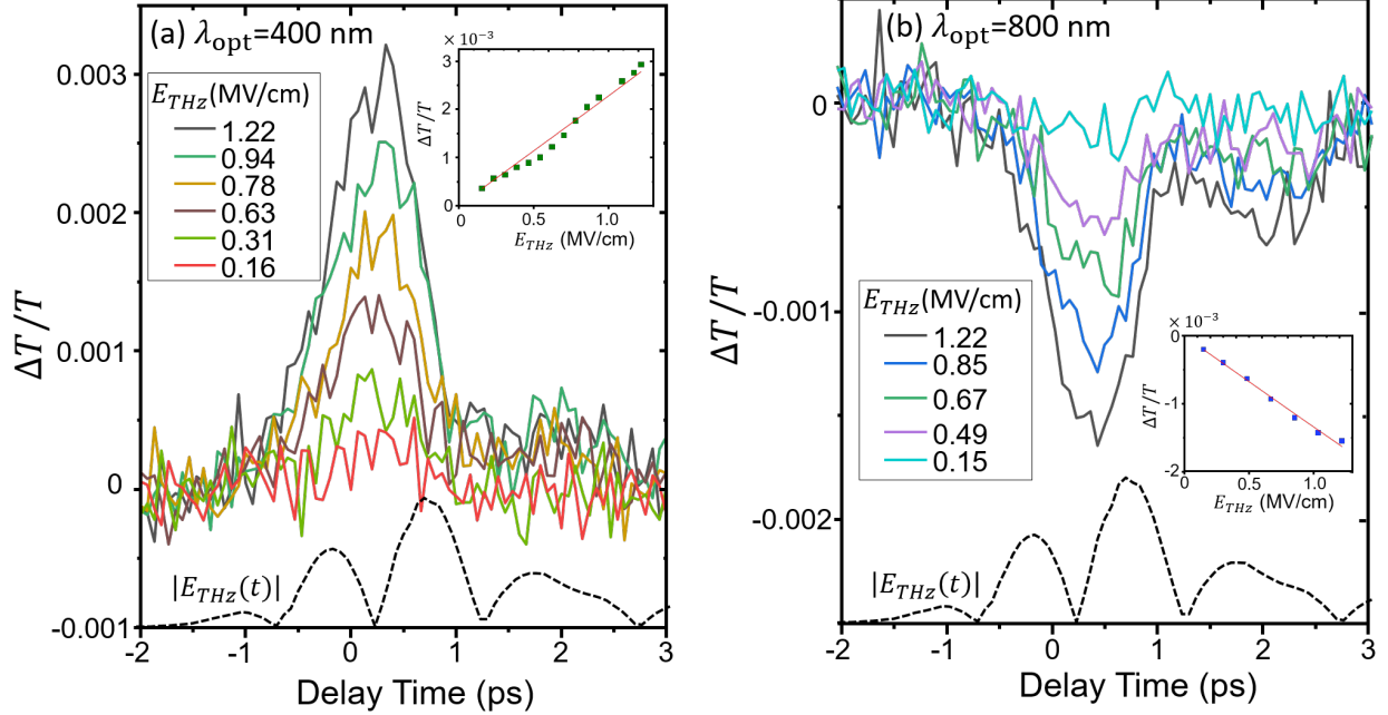
FIG. 2. Time-resolved differential transmission of optical probe pulses at (a) 400 nm and (b) 800 nm induced by intense THz fields. The peak THz field strength is varied from 0.15 MV/cm to 1.22 MV/cm. The insets show the maximum differential transmission vs. the peak THz field intensity. The dotted lines at the bottom presents the THz field magnitude as a function of the delay time.
