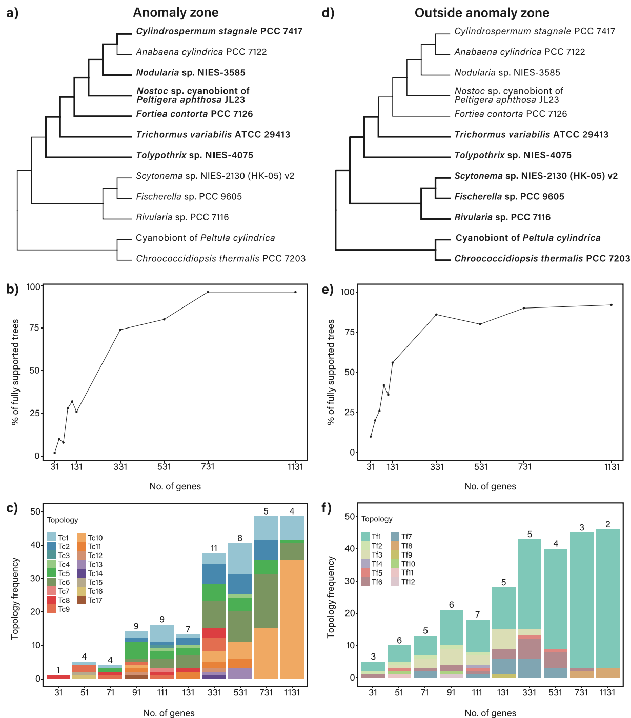
FIGURE 5. Phylogenetic support for relationships linked to the anomaly zone based on concatenated jackknife sets of increasing number of genes. The jackknifed gene sets were sampled from the amino acid L1648+ng alignments of taxa subset 1 (Table 2). We sampled 50 jackknife replicates for each number of genes. All trees were inferred using the site-heterogeneous model LG+PMSF.C60+G4+F and 1000 UFBoot replicates. Trees were trimmed to include only the lineages whose relationships (a) span the anomaly zone (thick branches and bold taxon names), or (d) that were outside the anomaly zone (thick branches and bold taxon names). (b) Percentage of anomaly zone subtrees inferred from jackknife sets of increasing number of genes where all internodes were highly supported (UFBoot > 95%). (e) Percentage of non-anomaly zone subtrees inferred from jackknife sets of increasing number of genes were all internodes where highly supported (UFBoot > 95%). (c) Distribution of distinct, fully supported topologies (i.e., all internodes with UFBoot > 95%) of subtrees in the anomaly zone. (f) Distribution of distinct, fully supported topologies (i.e., all internodes with UFBoot > 95%) of subtrees outside the anomaly zone. Two topologies were considered distinct if the Robinson-Foulds distance was > 0. Numbers above each bar indicate the number of distinct topologies. All topologies referenced in panels c and f are shown in Supplementary Figure S8.
