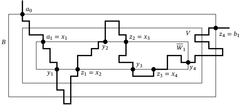
FIGURE 5.5. The path segment \pi_{a_0, b_1}^*(x) with four excursions \pi^1, \dots, \pi^4 . The segment \pi^{i,1} inside \bar{W}_1 goes from x_i to y_i and the segment \pi^{i,2} outside \bar{W}_1 goes from y_i to z_i . Note that \bar{W}_1 is not actually a box but is represented as one above for the purpose of illustration.
