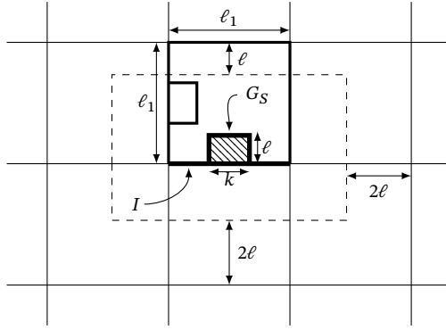
FIGURE 5.4. The proof of Lemma 5.9. The light grid is W_1 . The thicker square and its two detours are part of W_1 . The thickest edge of the square is denoted by I . The hashed box, denoted by G_S , is a detour rectangle attached to I . The points that are within distance \ell_1 - 2\ell from a point on I \cup G_S are all inside the dashed rectangle. All these points that are also on W_1 can be reached from any point on I via an \ell^1 path that stays on W_1 .
