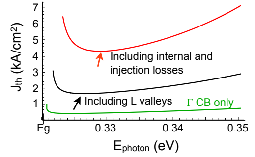
Fig. 4. Contributions to threshold current for DH GeSn laser. Populated L valleys add free carrier absorption, amplifying the effects of other losses. GeC(Sn) thresholds (not shown) remain entirely below the green bottom line.
