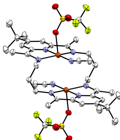
Figure 2. Crystal structure of ^3[\text{Cu}_2(\text{NCMe})_2]^{4+} (thermal ellipsoids set at 50% probability; hydrogen atoms, solvent molecules and outersphere anions omitted for clarity).
