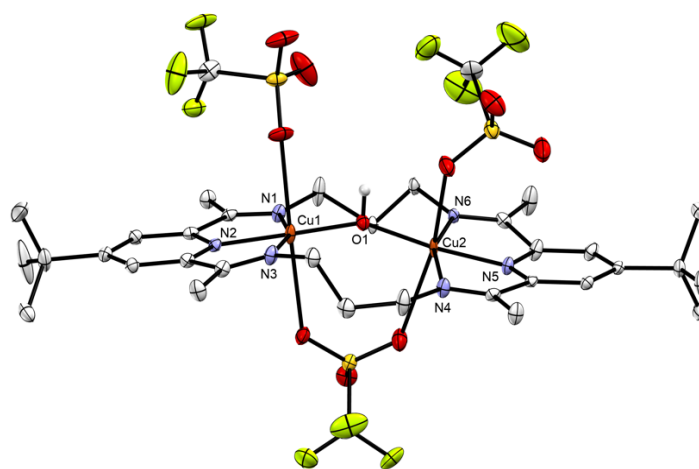
Figure 10. Crystal structure of 3 [Cu 2 OH] 3+ (thermal ellipsoids set at 50% probability; hydrogen atoms, solvent molecules, triflate disorder and macrocycle disorder omitted for clarity).
