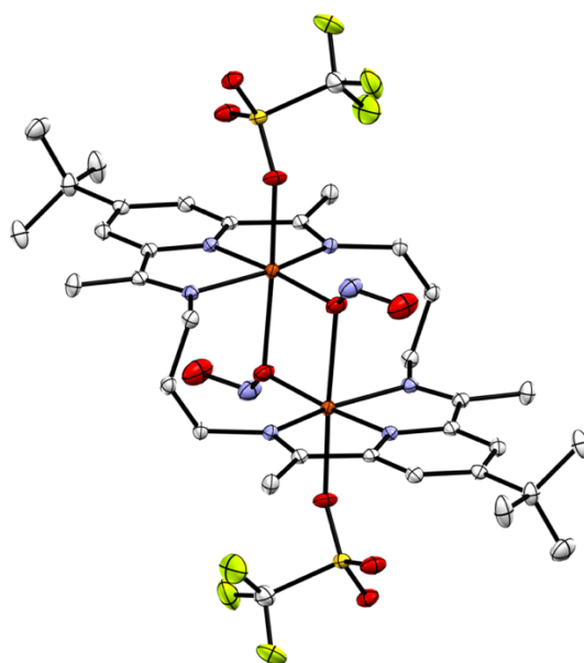
Figure 7. Crystal structure of ^3[\text{Cu}_2(\text{ONO})_2]^{2+} (thermal ellipsoids set at 50% probability; hydrogen atoms and nitrite disorder omitted for clarity).
