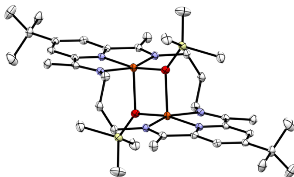
Figure 9. Crystal structure of ^3[\text{Cu}_2(\text{OTMS})_2]^{2+} (thermal ellipsoids set at 50% probability; hydrogen atoms and outer-sphere anions omitted for clarity).
