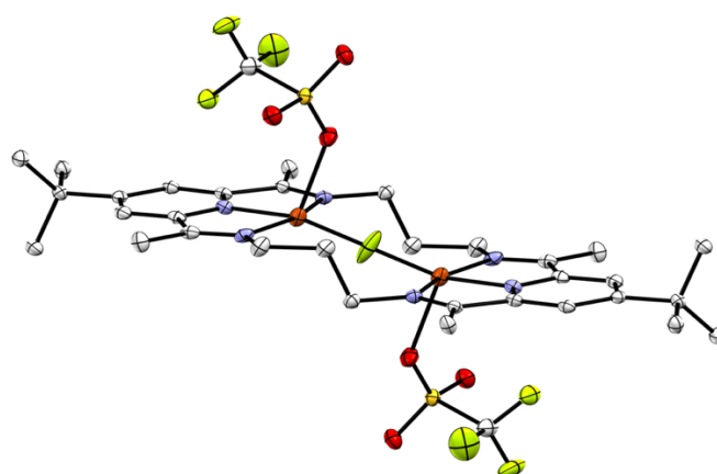
Figure 4. Crystal structure of ^3[\text{Cu}_2\text{F}]^{3+} (thermal ellipsoids set at 50% probability; hydrogen atoms, triflate disorder, and outer-sphere anions omitted for clarity).
