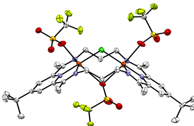
Figure 3. Crystal structure of ^3[\text{Cu}_2\text{Cl}]^{3+} (thermal ellipsoids set at 50% probability; hydrogen atoms and triflate disorder omitted for clarity).
