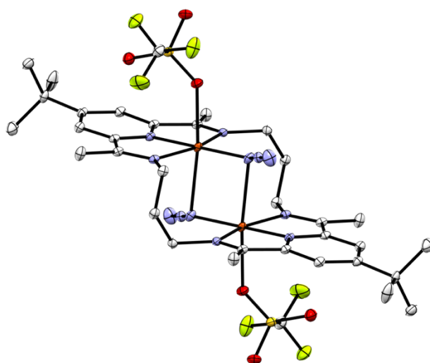
Figure 5. Crystal structure of ^3[\text{Cu}_2(\text{N}_3)_2]^{2+} (thermal ellipsoids set at 50% probability; hydrogen atoms omitted for clarity).
