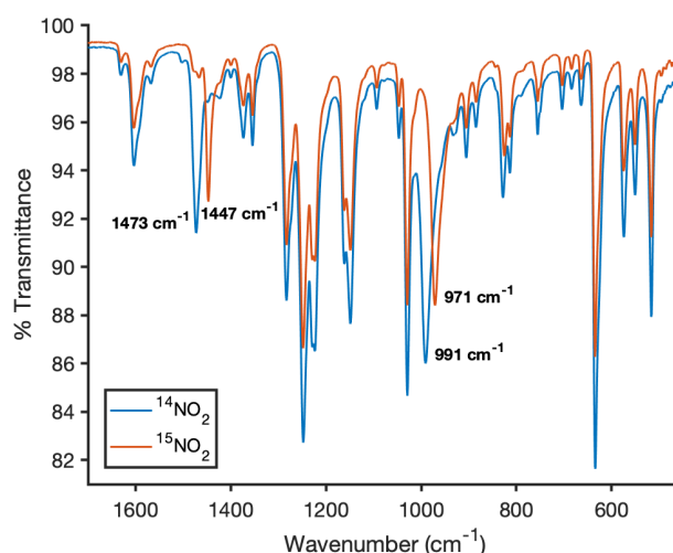
Figure 8. Overlay of infrared spectra of ^3[\text{Cu}_2(\text{O}^{14/15}\text{NO})_2]^{2+} .
