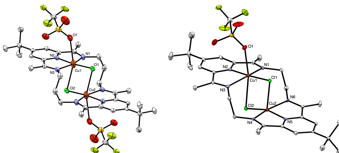
Figure 2. Left: Crystal structure of 3[\text{Cu}_2\text{Cl}_2]^{2+} (thermal ellipsoids set at 50% probability; hydrogen atoms and triflate disorder omitted for clarity). Right: Crystal structure of 2[\text{Cu}_2\text{Cl}_2]^{2+} (thermal ellipsoids set at 50% probability; hydrogen atoms, solvent molecules and outer-sphere anions omitted for clarity; one macrocycle of the asymmetric unit shown).
