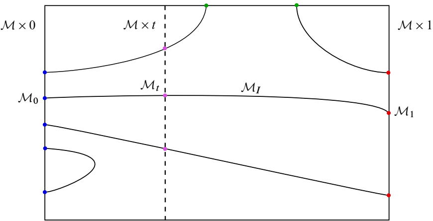
Figure 9: A schematic of the space \mathcal{M} \times I with \mathcal{M}_I inside it. Vertical slices of the picture such as the vertical dashed line represent the spaces \mathcal{M} \times t , while the solid curves collectively represent the smooth moduli space \mathcal{M}_I . The left and right endpoints on \mathcal{M}_I represent \mathcal{M}_0 \subset \mathcal{M} \times 0 and \mathcal{M}_1 \subset \mathcal{M} \times 1 respectively, while the endpoints of \mathcal{M}_I on the top and bottom of the figure represent degenerations of triangles into broken triangles in the compactification.
