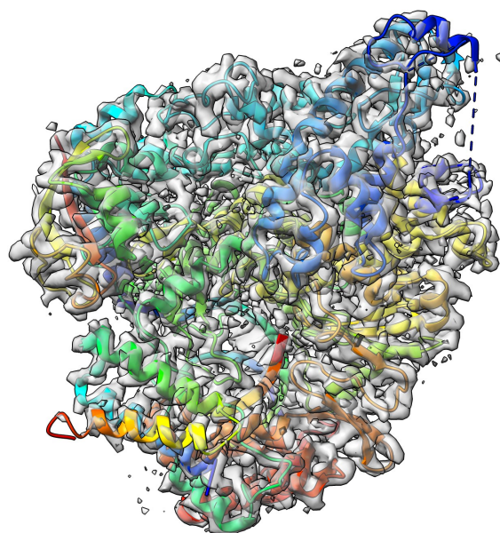
Figure 4. Target 202 (EMD-30210) map-model overlay at the recommended contour 0.058 (4.3 s) with T0202EM004_1 (ours).
