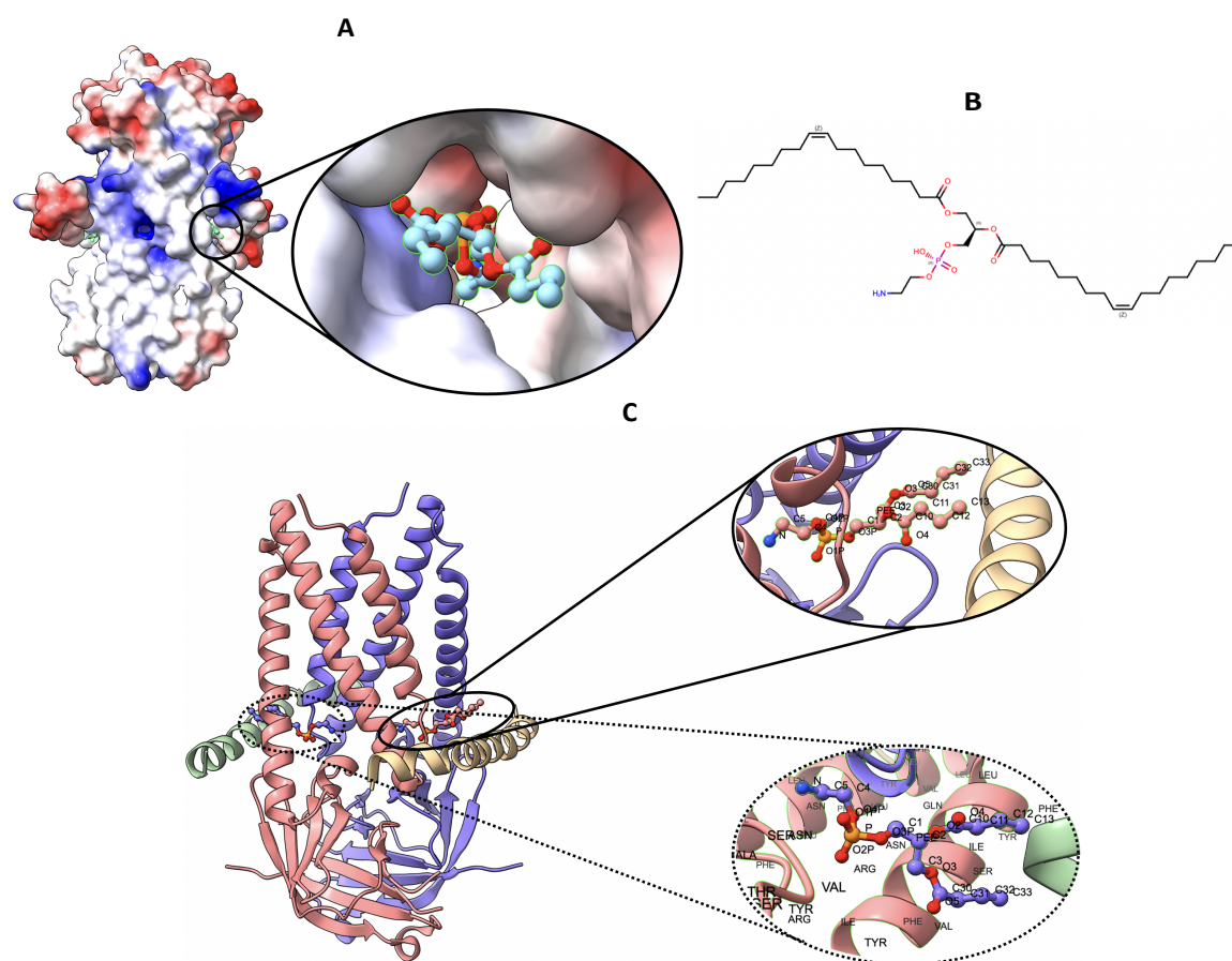
Figure 8. Target 203. (A) T0203EM0004_1 (ours) docked by Target 203 (EMD-22898) and visualized with electrostatic potential surface generated in UCSF Chimera. (B) Ligand PEE, image extracted from Protein Data Bank (PDB). (C) Protein–ligand interactions in T0203EM0004_1 (our) model. Chains are colored differently (chain A: blue, chain B: pink, chain C: green, and chain D: golden). The ligand are labeled with their atom names as well as the ligand’s name (PEE).
