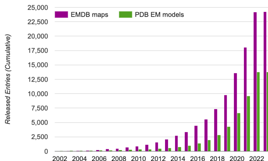
Figure 1. The growth of cryo-EM density maps and cryo-EM-derived protein structures. The statistics were obtained from EMDataResource [34], a unified data resource for 3-Dimension electron microscopy (3DEM) on 20 November 2022.
