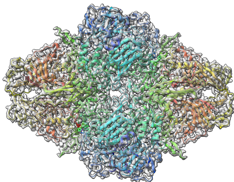
Figure 3. Target 201 (EMD-7770) map-model overlay at the recommended contour 0.52 (3.3 s) with T0201EM0004_1 (ours).
